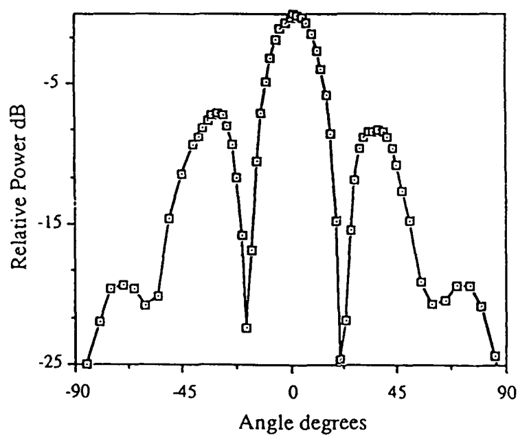
H-Plane Radiation Patteren
