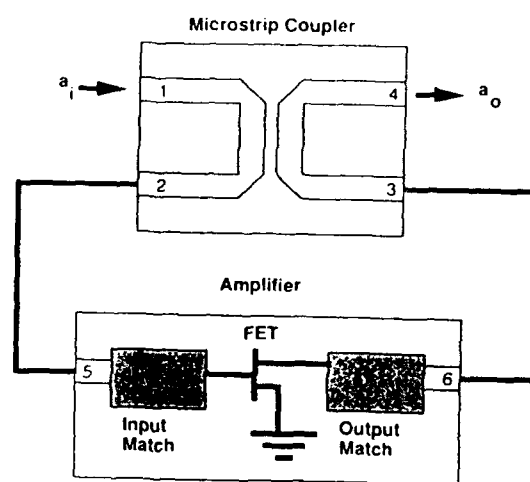
Schematic diagram of two port oscillator.
