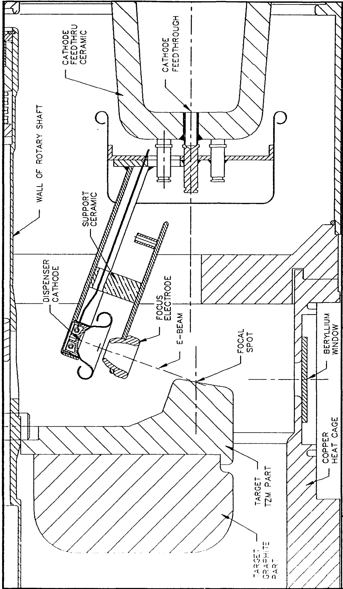
Figure 14. Final electron gun design mounted in X-ray tube
