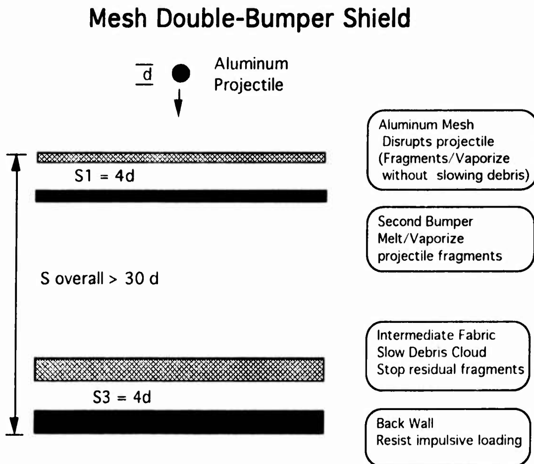
Figure 55. Mesh Double Bumper 40
