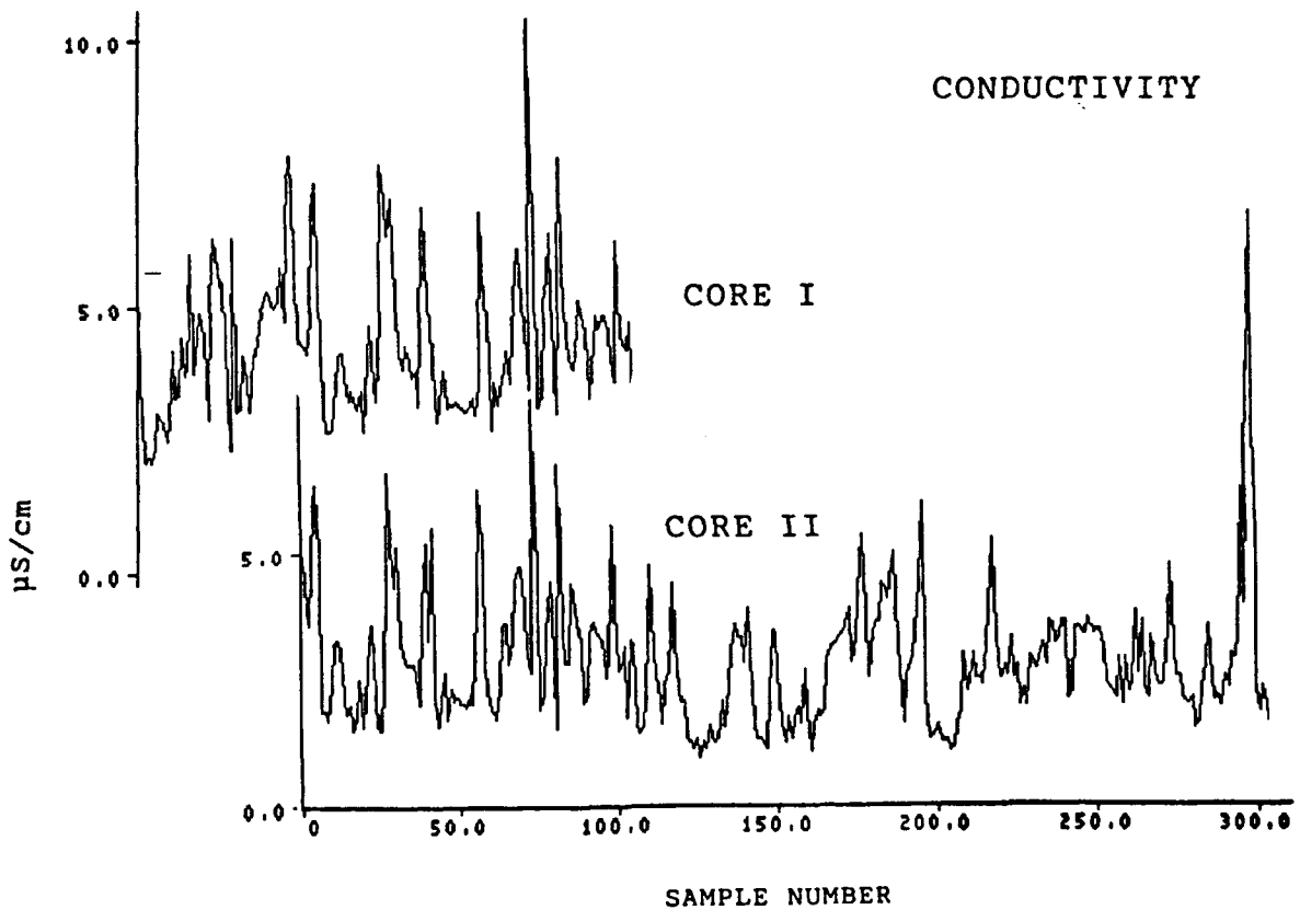
Figure 2. Nitrate concentration and liquid conductivity records from two cores that overlap about two meters and were drilled about half a meter apart.
