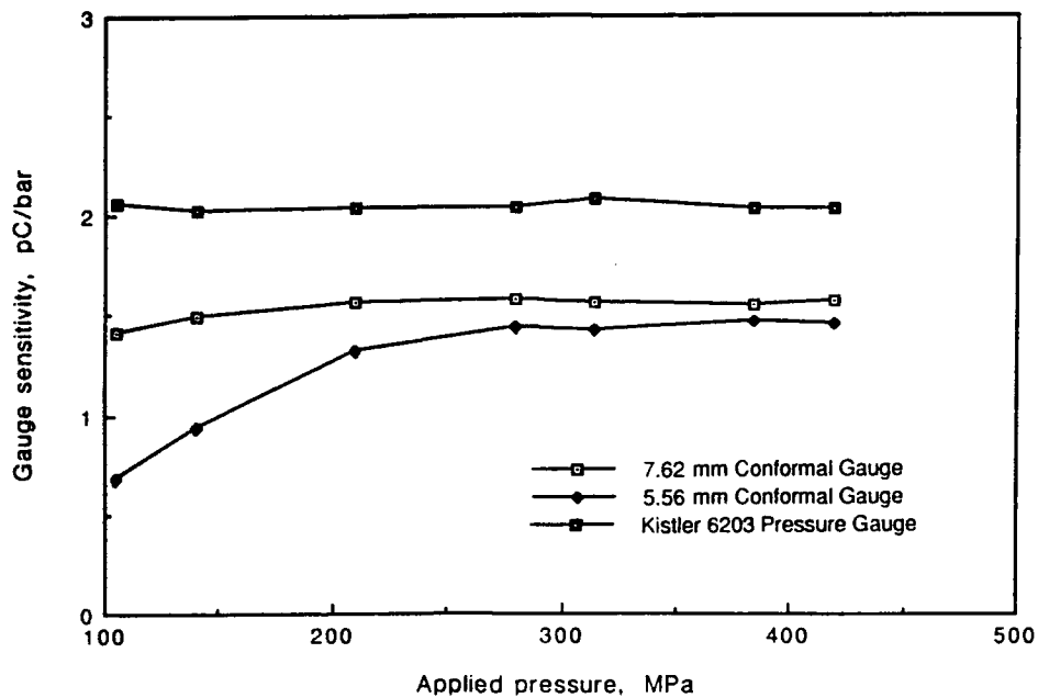
Figure 5: Transducer Linearity.
