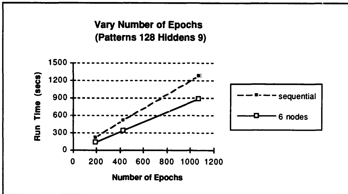
Figure 42. Vary Number of Epochs
