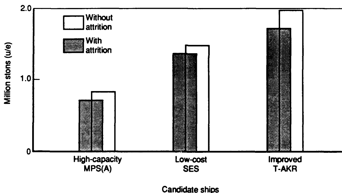
Fig. 6—Cumulative cargo deliveries over 90 days (Europe, zero warning, with and without ship attrition)
