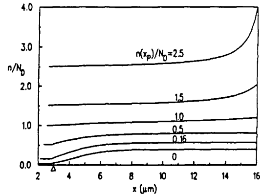
Fig. 7. Electron concentration in the space charge region.
