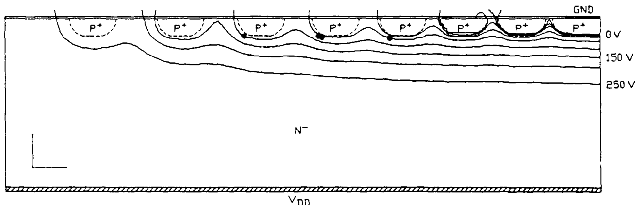
Fig. 7 Potential distribution for seven-ring termination structure ( N_{ss} = 0 , V_{BD} = 281 \text{ V} ).
