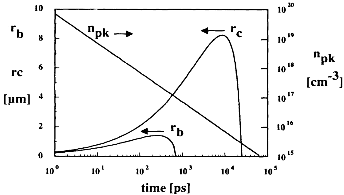
Figure 4: Radii of core regions corresponding to and and peak carrier concentration of the plasma filament resulting from a 150MeV Fe ion.
