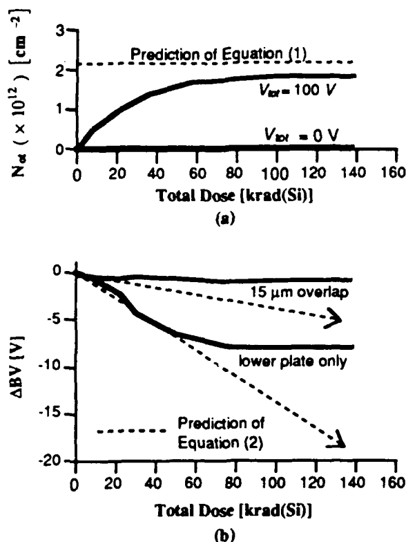
Figure 3. Comparison of experimental data (heavy lines) and predicted response (dashed lines). (a) N_{ox} vs. D for device of figure 2a. (b) \Delta BV vs. D for devices of figure 2b.
