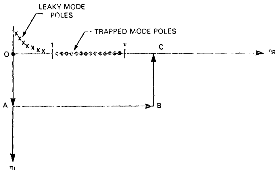
FIGURE C-1. CONTOUR OF INTEGRATION TO EVALUATE THE FUNCTION P_{nm}
