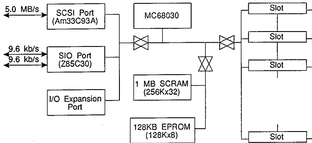
Figure 3.1: Block Diagram of the InvestiGATOR Array Processor Testbed
