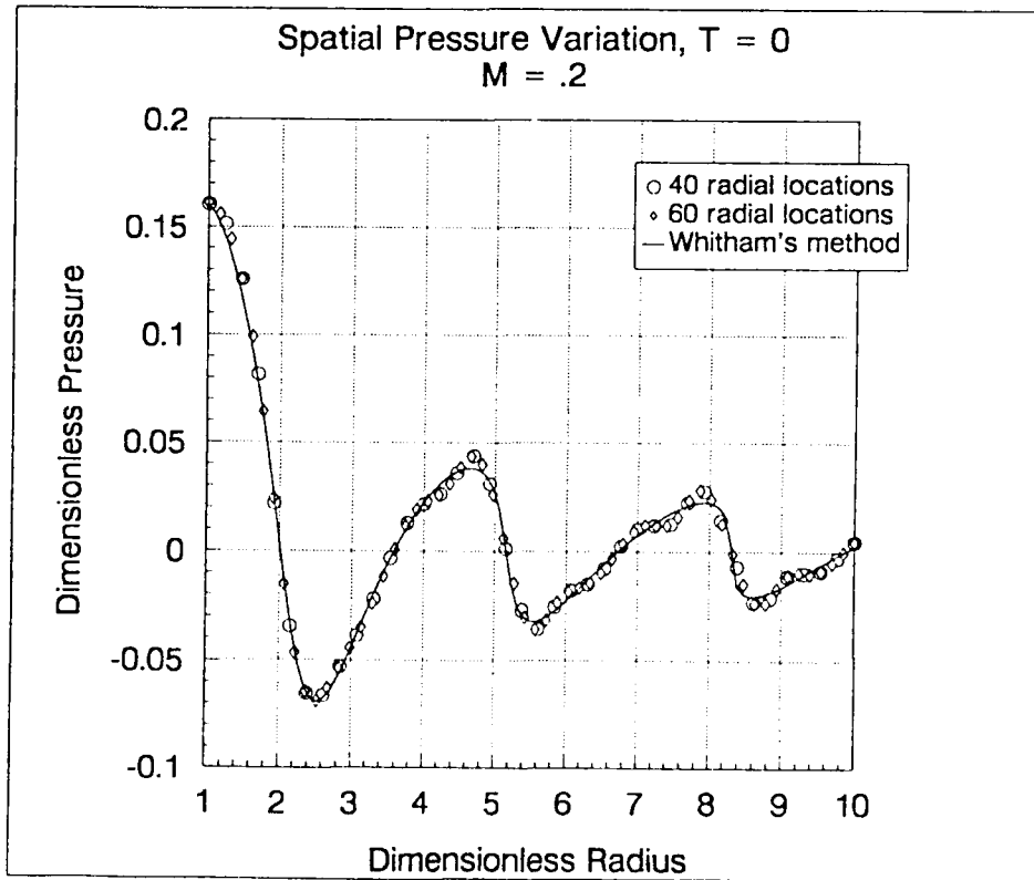
Figure 8: Solution at t = 0 for four Fourier terms.
