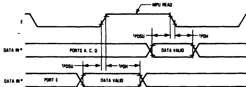
Figure 11-10. Port Read
