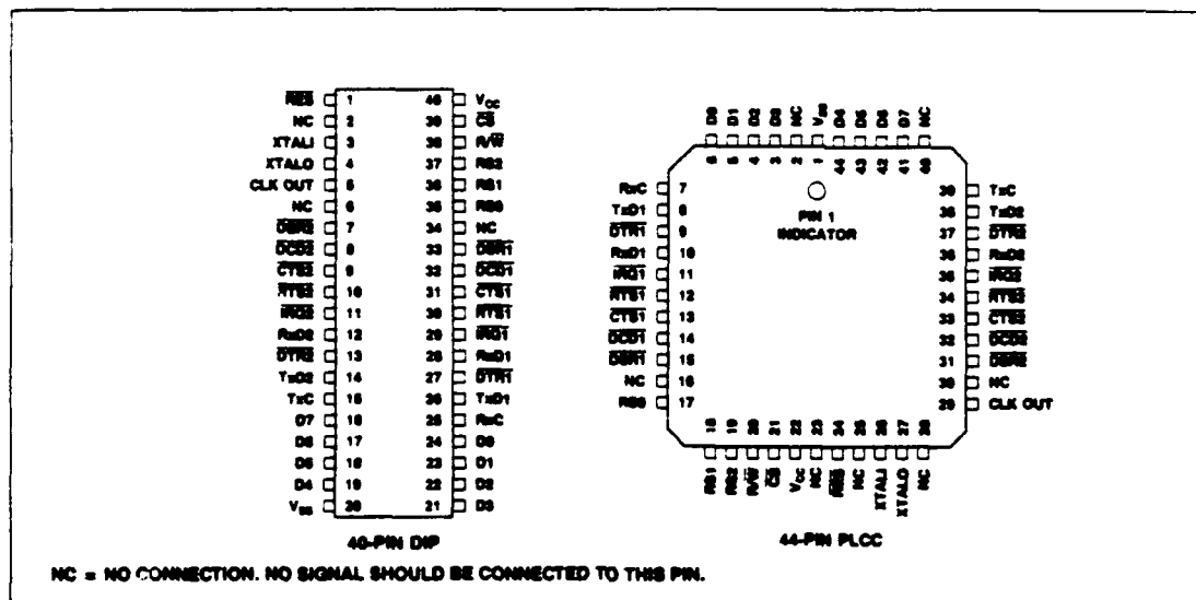
Figure 1. R65C52 Pin Assignments
