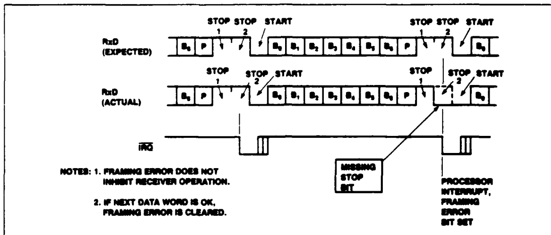
Figure 15. Framing Error
