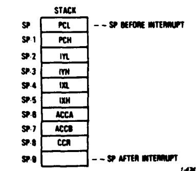
Figure 2-2. Interrupt Stacking Order
