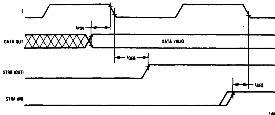
Figure 11-14. Port C Output Handshake
