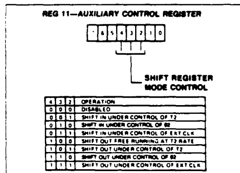
Figure 21. Shift Register Modes
