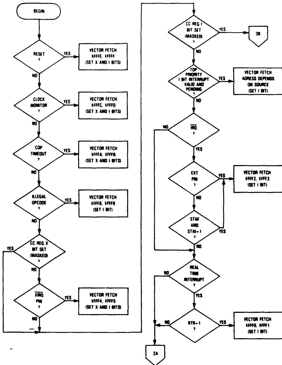
Figure 3-2. MC68HC11A8 Interrupt Structure Flowchart (Sheet 1 of 3)
