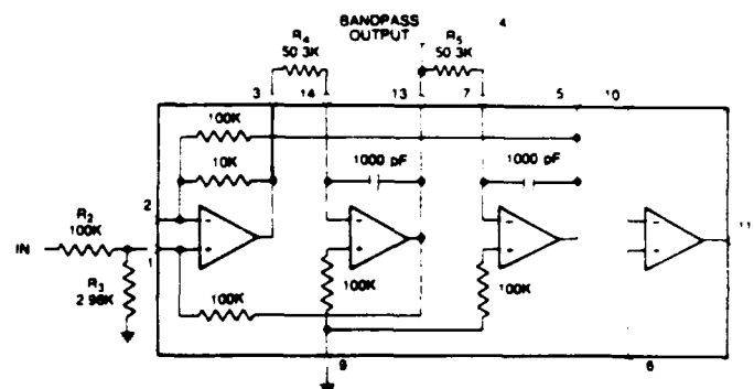
Figure 6. Bandpass Filter Example
