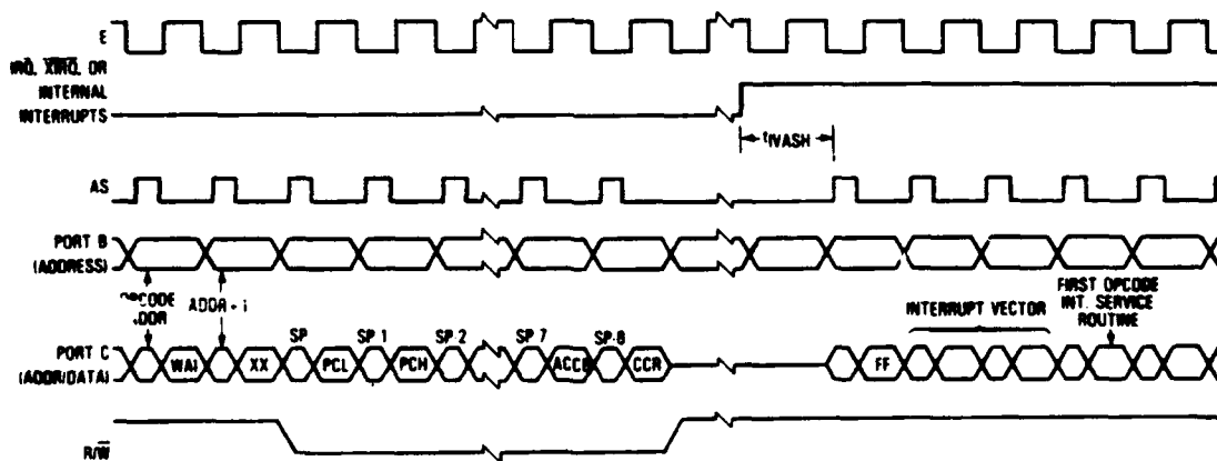
Figure 11-4. Wait Recovery From Internal or External Interrupts Timing Diagram
