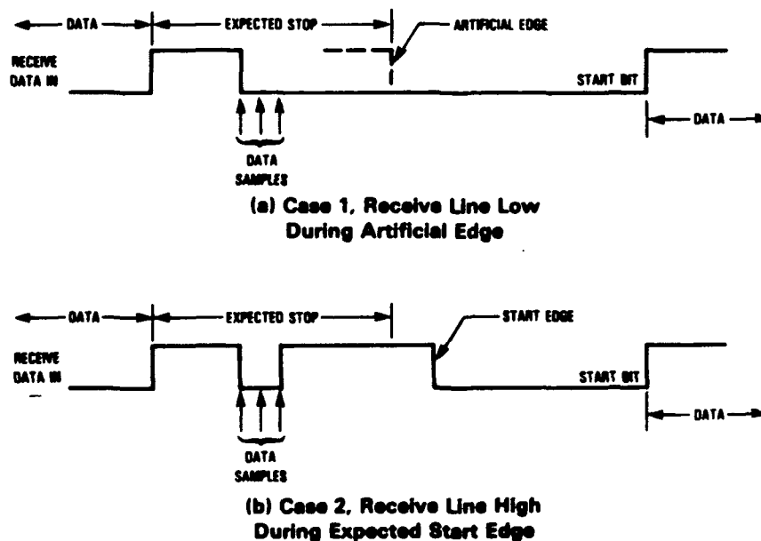
Figure 5-4. SCI Artificial Start Following a Framing Error
