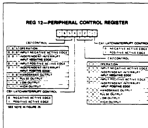
Figure 11. Peripheral Control Register (PCR)
