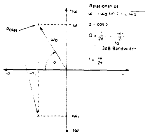
Figure 2. S-Plane Diagram
