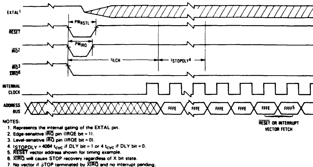
Figure 11-3. Stop Recovery and Power-On Reset Timing Diagram
