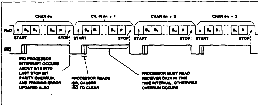
Figure 12. Continuous Data Receive
