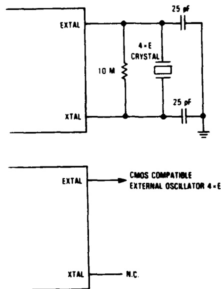
Figure 11-18. Oscillator Circuits
