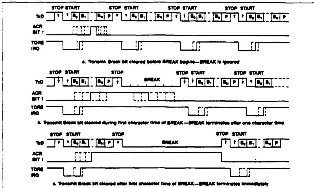
Figure 9. Transmit BREAK
