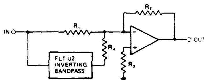
Figure 12. Realization of Notch Filter
