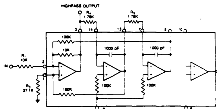
Figure 10. Highpass Filter Example
