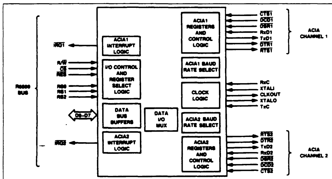
Figure 2. R65C52 DACIA Interface Signals
