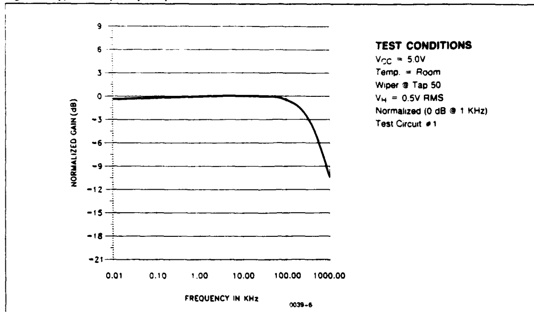
Figure 1: Typical Frequency Response for X9103
