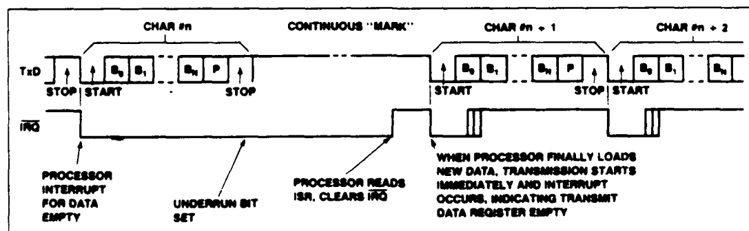
Figure 8. Transmit Underrun Condition Relationship
