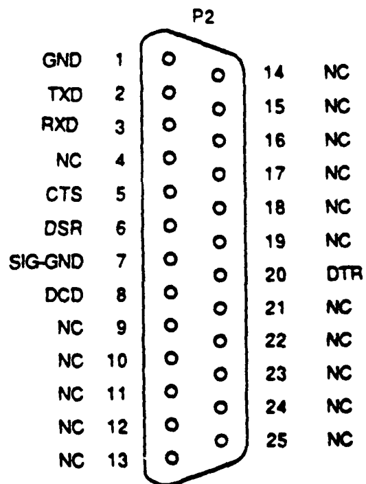
RS-232 Pin Assignment Diagram for the Host Port of the EVB
