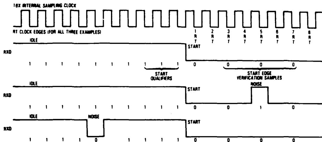
Figure 5-3. Examples of Start Bit Sampling Techniques
