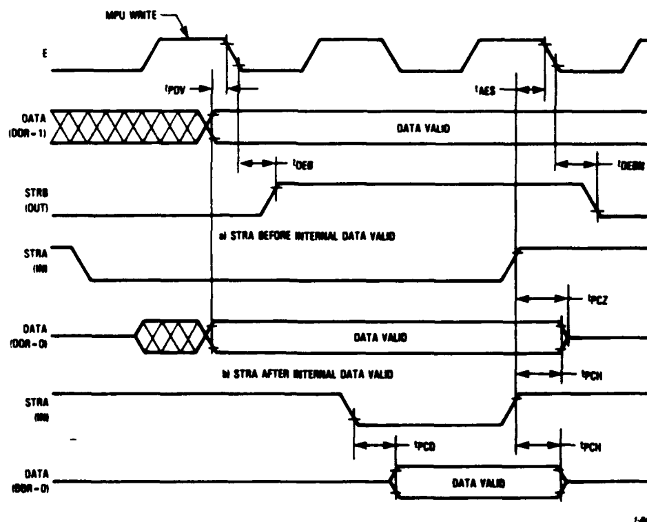
Figure 11-15. Port C Output Handshake with 3-State Enabled (STRA Enables Output Buffer)
