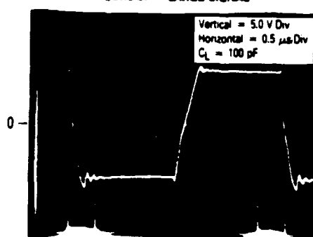
FIGURE 27 — LARGE-SIGNAL
