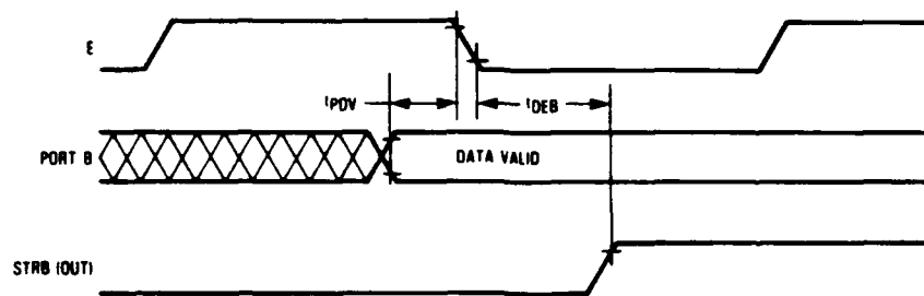
Figure 11-11. Simple Output Strobe
