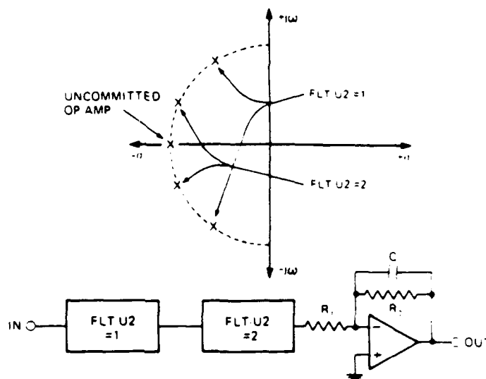
Figure 11. Realization of a Complex Multipole Filter
