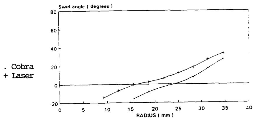
Fig 33 - Laser Anemometry Results and Cobra Probe Results at Window B (Flow angle, PR= 3.5)
