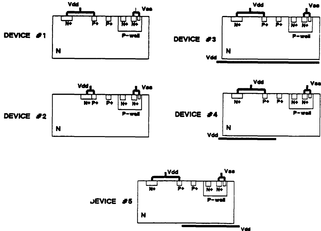
Figure 15: Inverter test structures utilized in the comparative study
