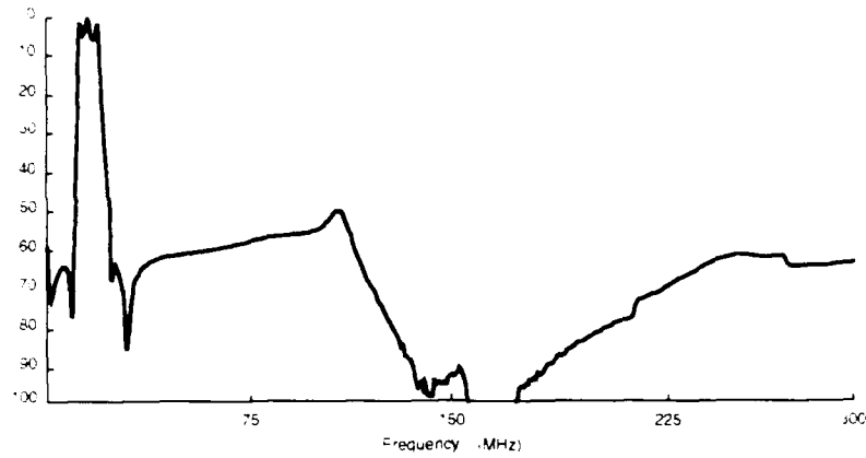
Figure 6. Magnitude Response - BPF : T-30-2
