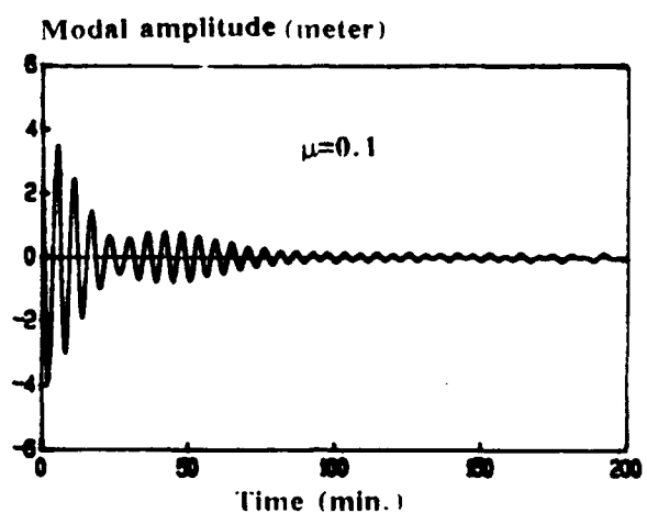
Fig. 5-4-4 Filtering observer
