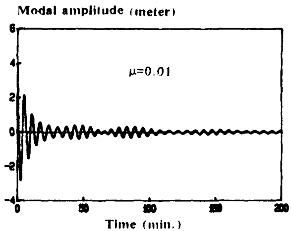
Fig. 5-2-6 Filtering observer
