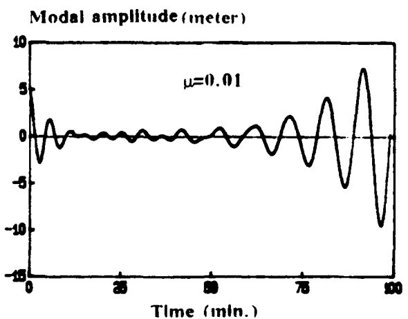
Fig. 5-4-5 Predicting observer
