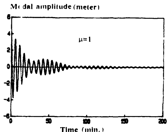
Fig. 5-2-2 Filtering observer
