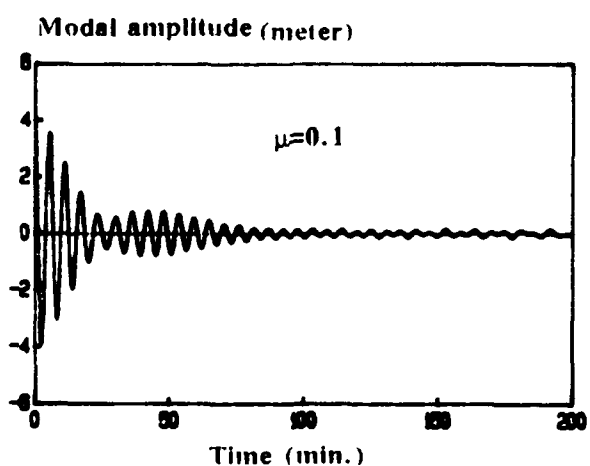
Fig. 5-4-3 Predicting observer
