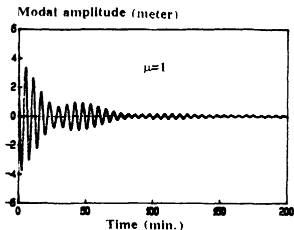
Fig. 5-2-1 Predicting observer
