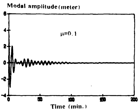
Fig. 5-2-4 Filtering observer
