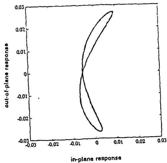
Figure 3 Periodic whirling response to parametric and external excitation
