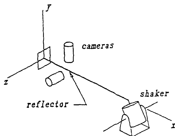
Figure 1 Experimental setup
