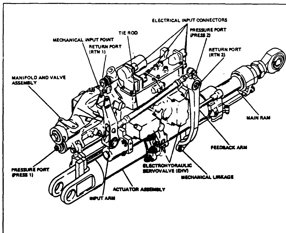
Figure C-1. Servocylinder Assembly.
