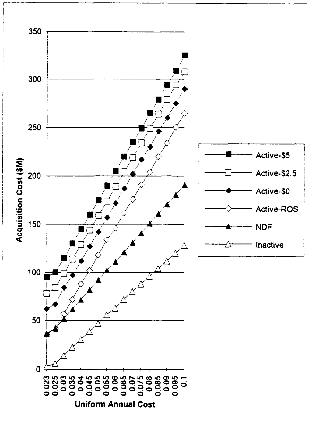
Figure 5. Acquisition Cost vs. Uniform Annual Cost (10% Discount Rate)
