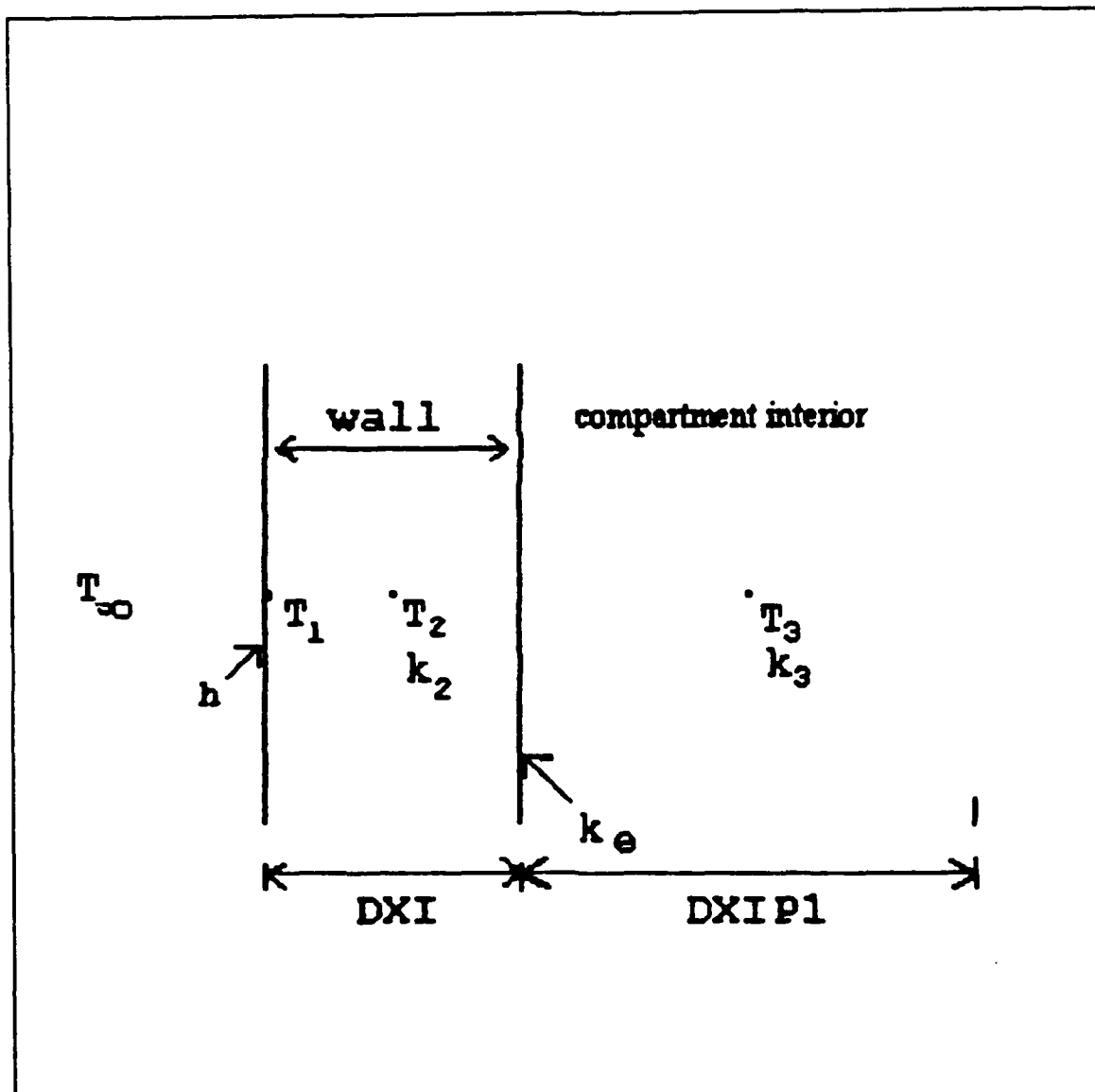
Figure 2.2 Conduction Model
