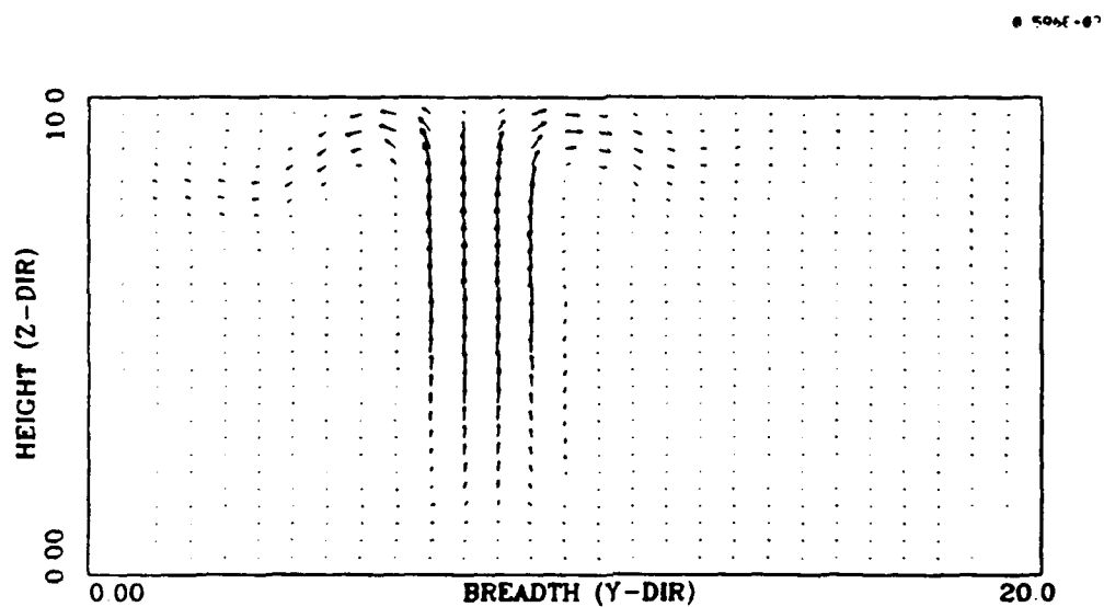
Y-Z ELEVATION (X = 17.00 FT.) AT 60.00 SEC.
