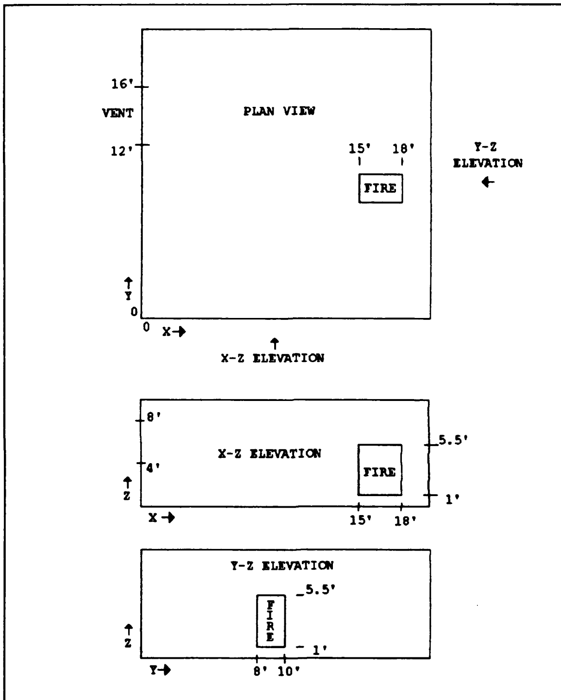
Figure 3.2 Graphics plots orientation
