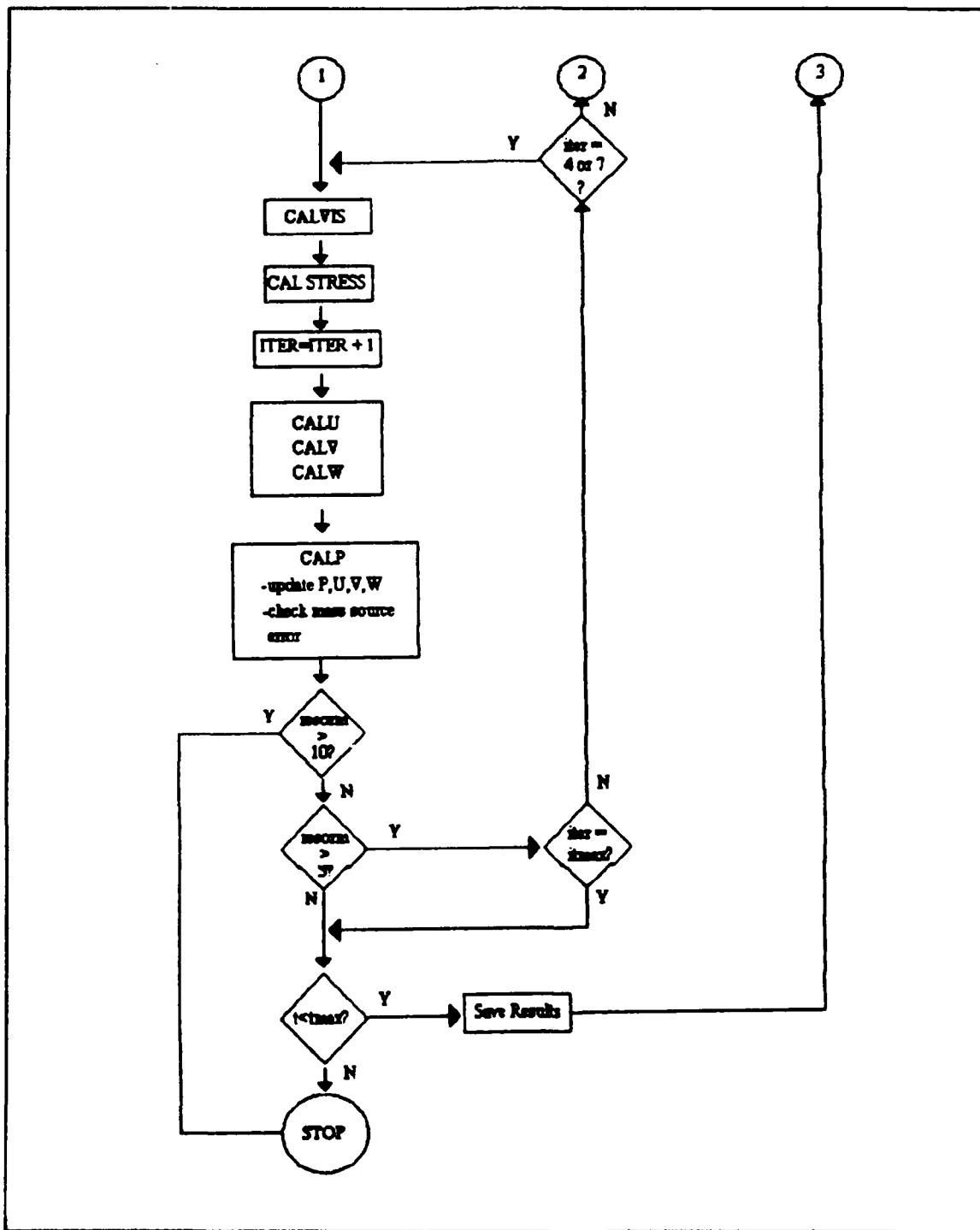
Figure A2 Program Flow Chart
