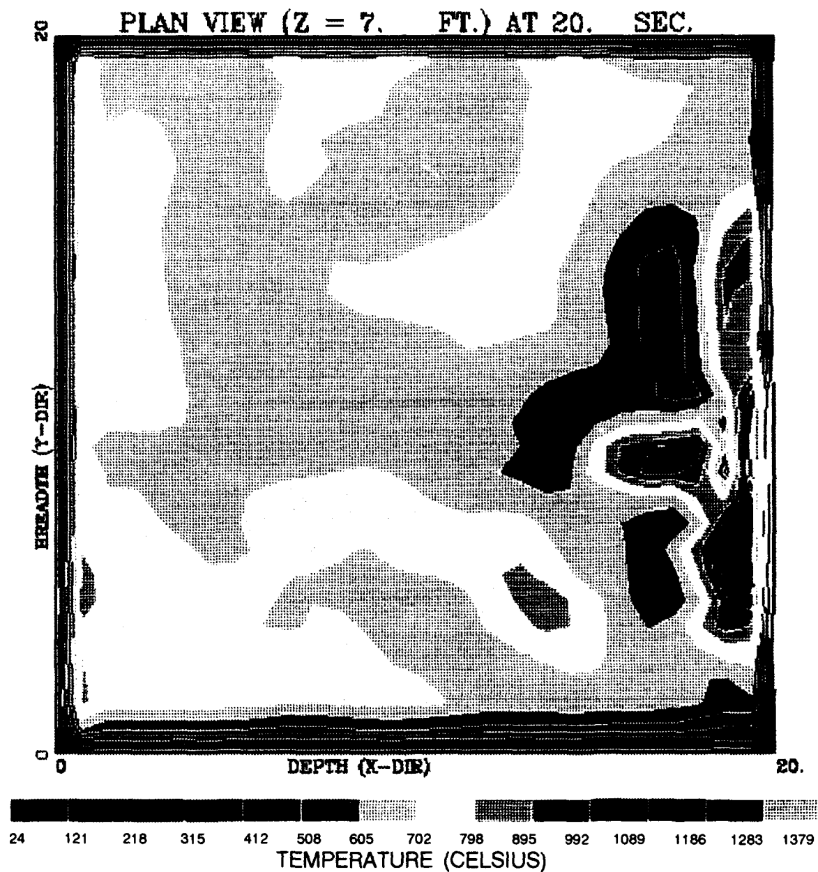
Figure 3.14 Trial 2 Isotherm Profile Plan View at 20s
