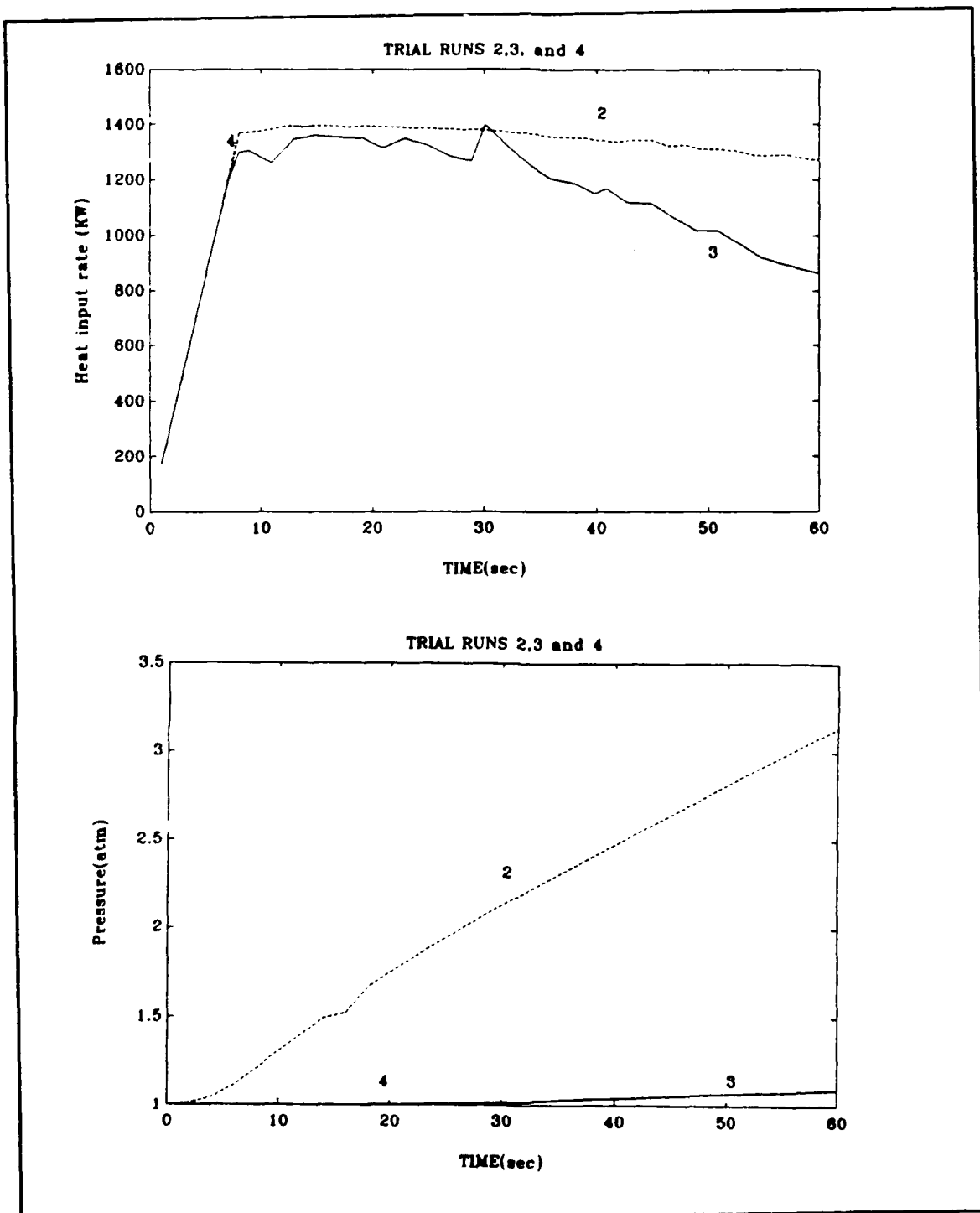
Figure 3.3 Trials 2,3,4 Heat Input/Pressure Curves
