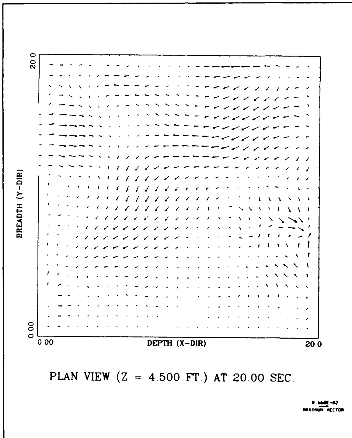
Figure 3.33 Trial 6 Velocity Profile Plan View at 20s
