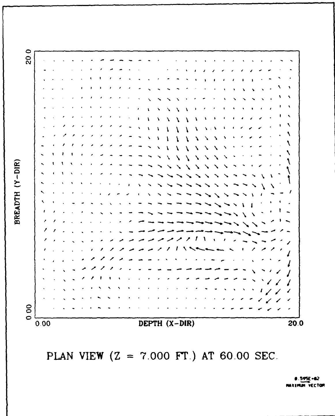
Figure 3.12 Trial 2 Velocity Profile Plan View at 60s
