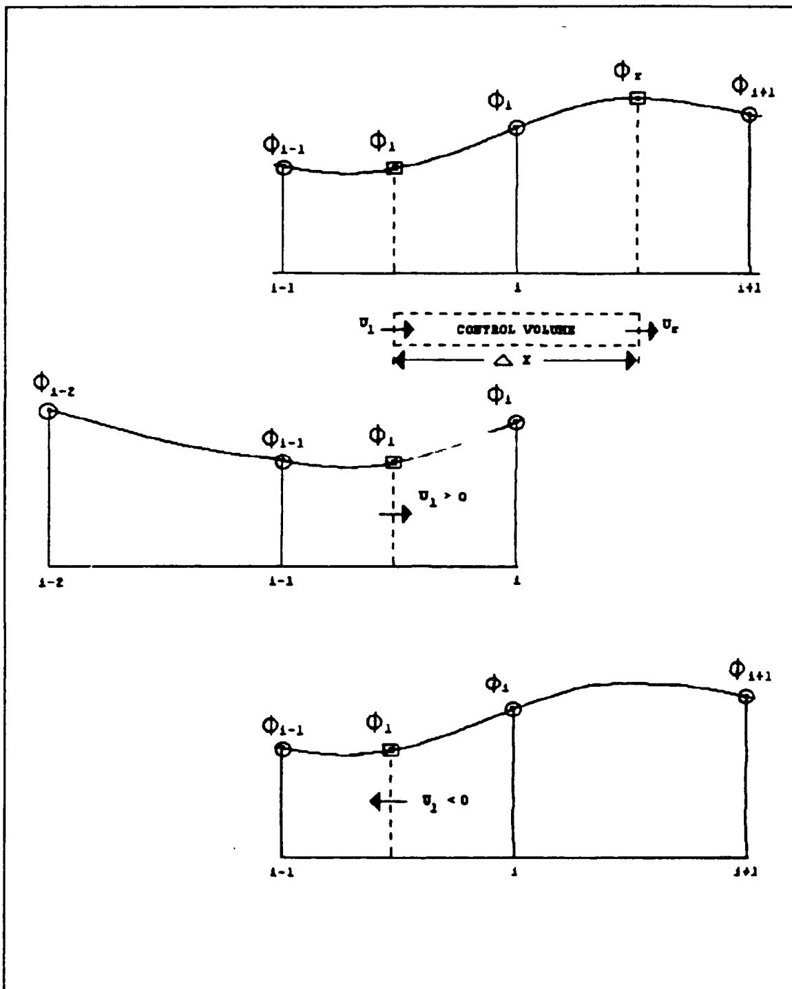
Figure 2.1 QUICK Scheme Portrayal
