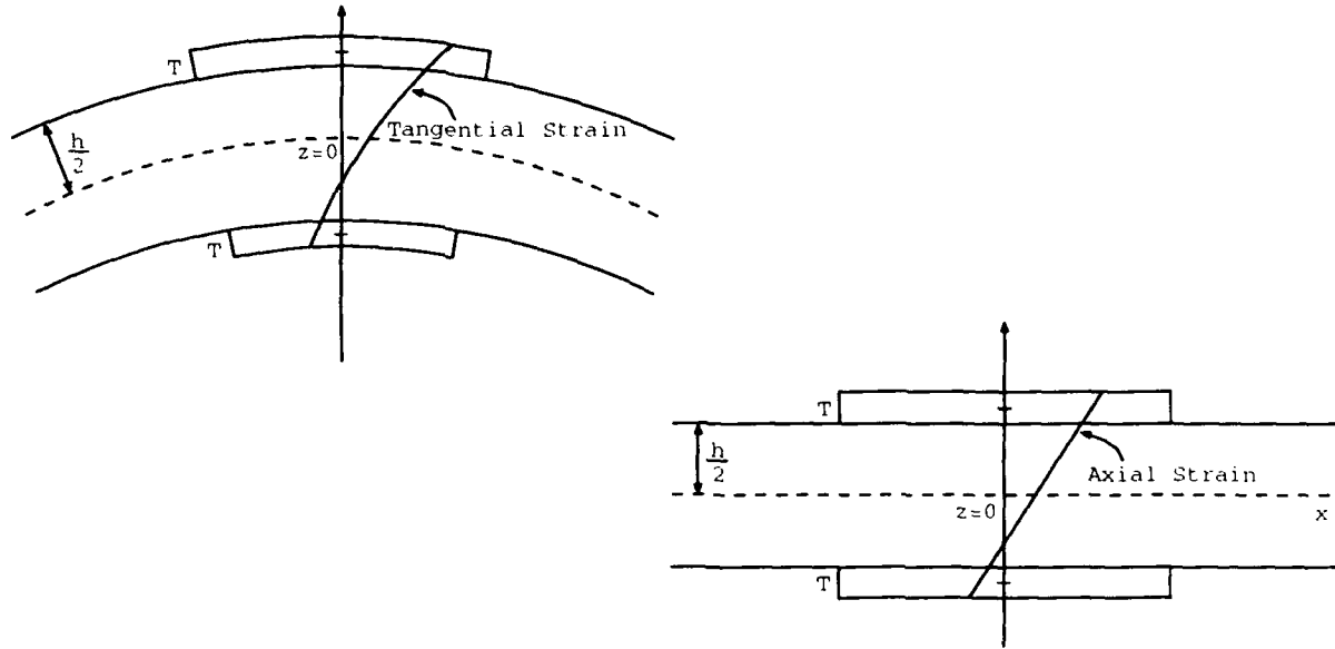
Figure 3. Strain Distribution for the Composite Structure.
