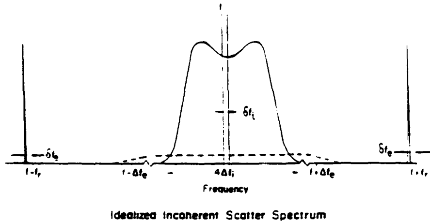
Figure 5-1: Incoherent scatter power spectrum when \lambda \gg \lambda_d . [after Rishbeth, 1989]
