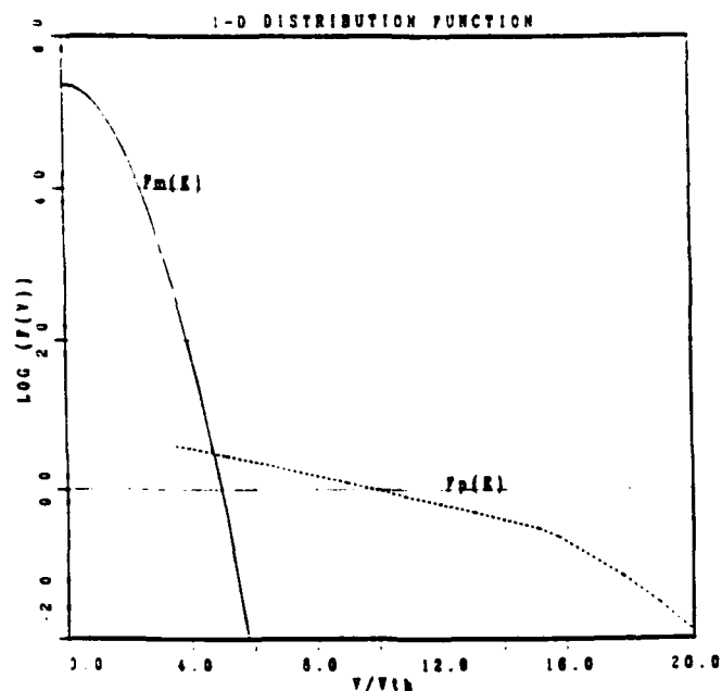
Figure 7-8: The 1-D electron distribution function used to calculate the enhanced Langmuir wave spectrum. The ordinate is in units of m^{-4}\text{sec} , while the abscissa is normalized by the electron thermal velocity, V_{te} .
