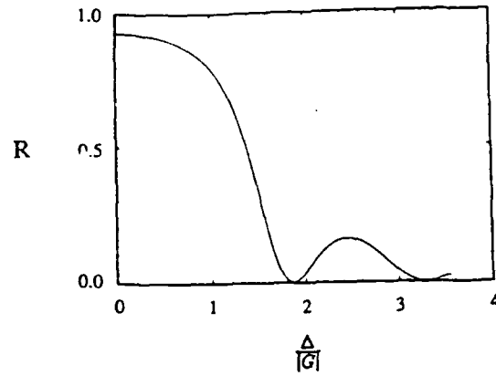
Fig. 2. Reflection coefficient from uncoupled mode theory for a section of corrugated waveguide with GL = 2 versus Bragg resonance mismatch.
