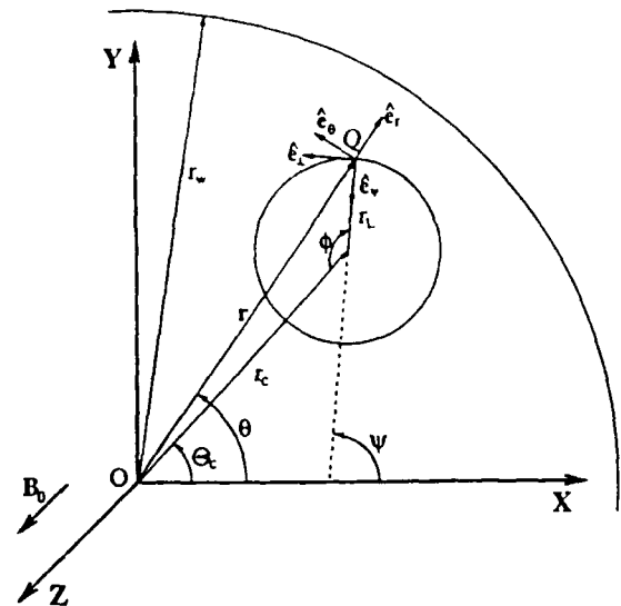
Fig. 1 Projection of equilibrium electron orbit on cross-sectional plane of waveguide in uniform magnetic field B_0 . Point O is the center of waveguide, r_w is the waveguide radius, point Q is the instantaneous position of the electron, r_L , r_c , and \theta_c are the electron Larmor radius, guiding center radius, and azimuthal angle, respectively, and r and \theta are real-space polar coordinates.
