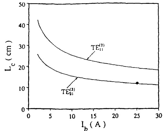
Fig. 4 Dependence of critical length on beam current for backward wave oscillations at second harmonic in TE_{11} mode and third harmonic in TE_{31} mode (100 kV, \alpha = 1 , r_c/r_w = 0.4 , r_w = 0.44 cm, B_0/B_g = 0.98 for TE_{11}^{(2)} plot and B_0/B_g = 1.15 for TE_{31}^{(3)} plot). Solid dot is from multimode particle simulation.
