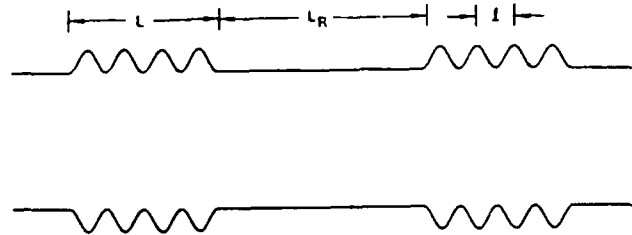
Fig. 1. Schematic of Bragg resonator with sinusoidal corrugation.
