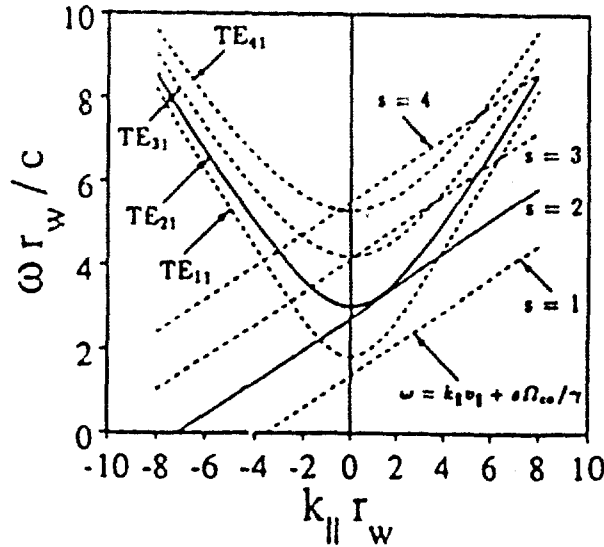
Figure 6: Uncoupled dispersion relation of operating mode (intersection of unbroken curves) and likely oscillating modes (intersections of broken curves with negative k_{||} ) for TE_{21}^{(2)} gyro-TWT amplifier (100 kV, \alpha = 1 , B_0 = 0.98B_g ).
