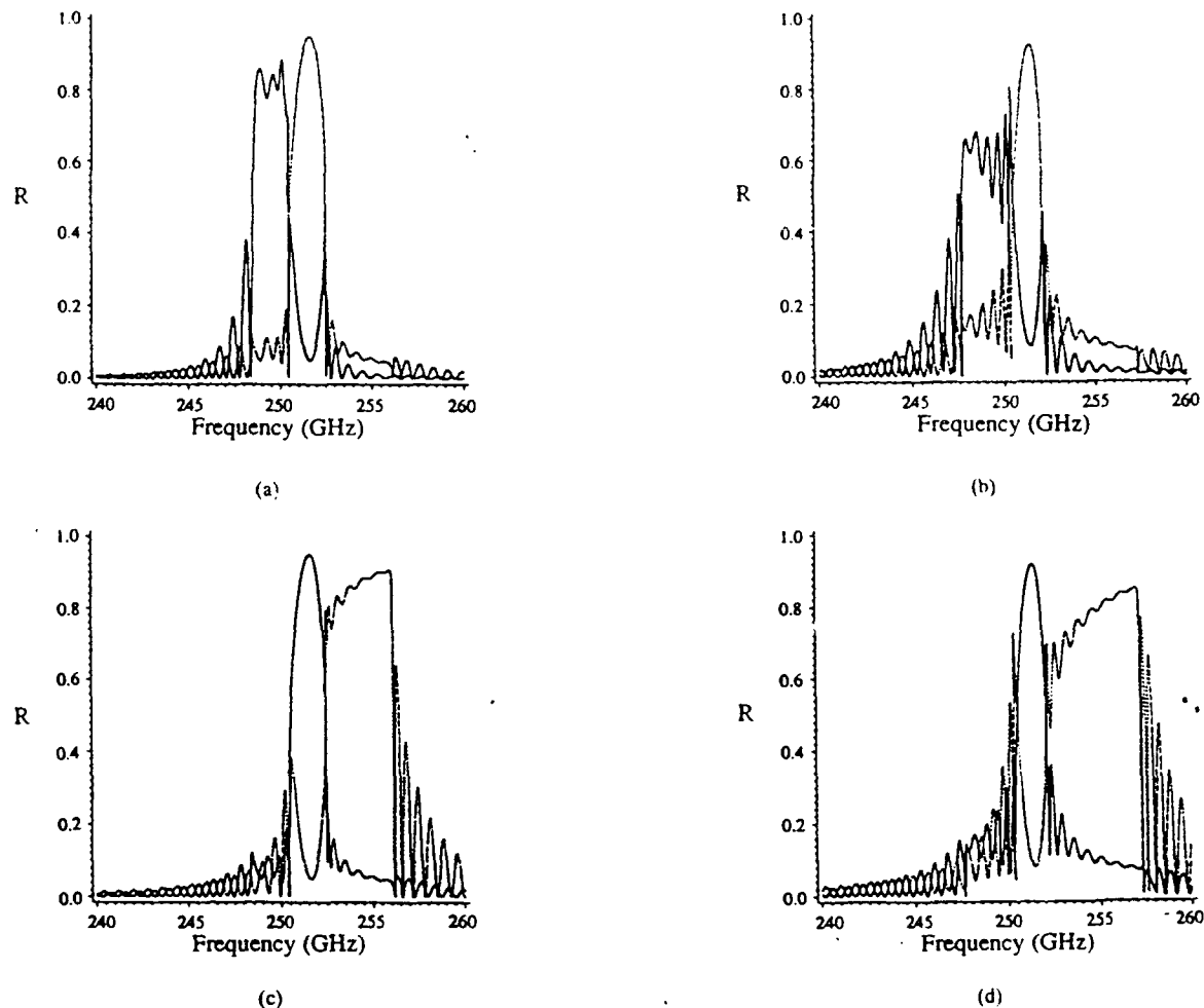
Fig. 3. Dependence on frequency of reflection in TE_{11} (solid line) and TM_{11} (dashed line) modes from sinusoidal corrugation reflector with parameters otherwise corresponding to those in Table I, case (a), with corrugation amplitudes of (a) 0.026 mm and (b) 0.039 mm for TE_{11} mode input and (c) 0.026 mm and (d) 0.039 mm for TM_{11} mode input
