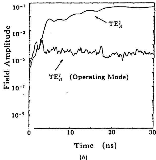
Figure 2. Field amplitudes of self-oscillating modes versus time in an unsevered interaction waveguide of 15cm in length for (a) Case a and (b) Case b (superscript indicates cyclotron harmonic number).
