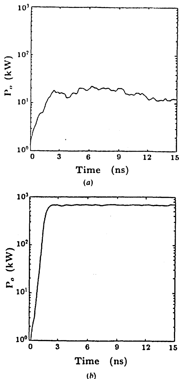
Figure 5. Temporal growth of TE 21 drive wave for Case b due to (a) spoiled beam of Figs 3(b) and 4(b) and (b) good quality beam.
