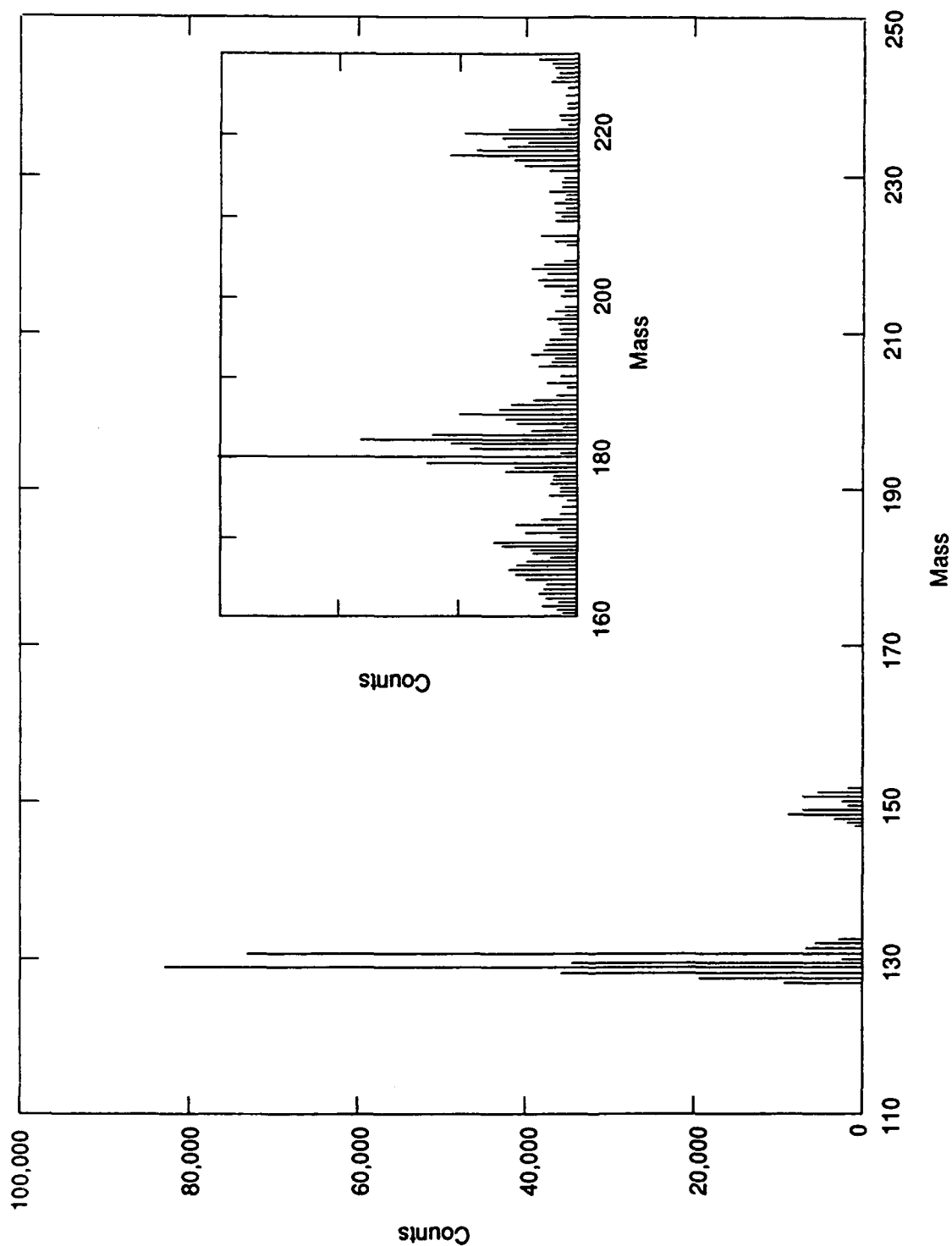
Figure 13. Mass Spectrum of a 1:20 Mixture of \text{CF}_3\text{Br} in \text{O}_2 at 700 \text{ \AA} ( 17.71 \text{ eV} ). (The nozzle stagnation pressure was 1741 \text{ torr} and the mass range displayed is m/e = 110 to 250 . The inset gives the expanded scale portion over the mass range of m/e = 160 to 230 .)
