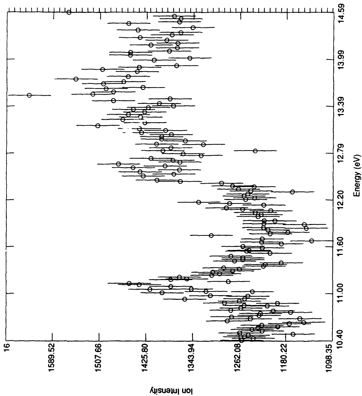
Figure 9. Autoionization Structure in \text{C}_6\text{H}_6 \cdot \text{O}_2 + h\nu \rightarrow (\text{C}_6\text{H}_6 \cdot \text{O}_2)^+ + \text{e}^- .
