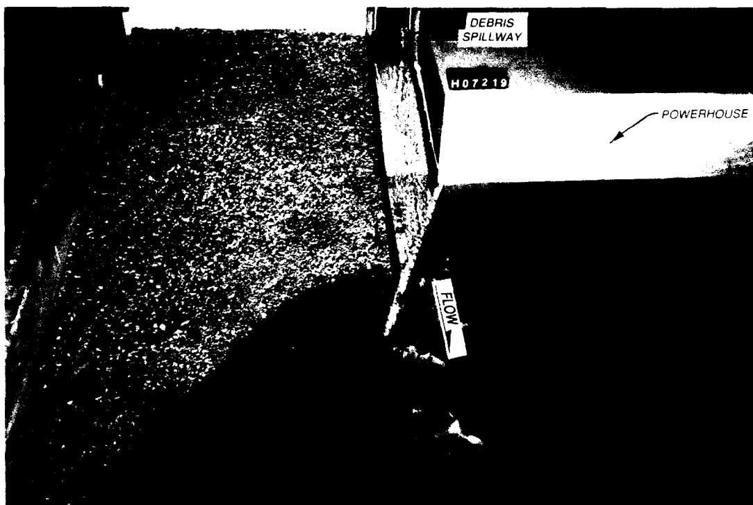
Photo 8. Flow conditions, type 3 design, discharge 2,640 cfs; pool el 80.8; tailwater el 40.0
