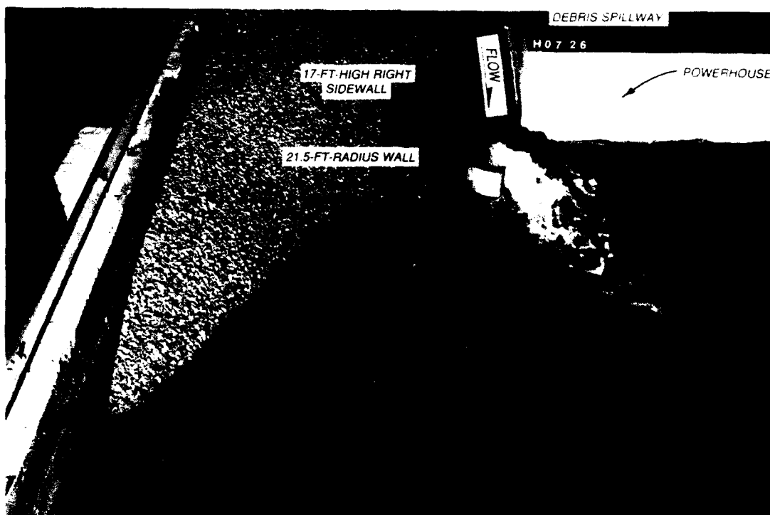
Photo 19. Flow conditions, type 17 design; discharge 2,640 cfs; pool el 80.8; tailwater el 40.0
