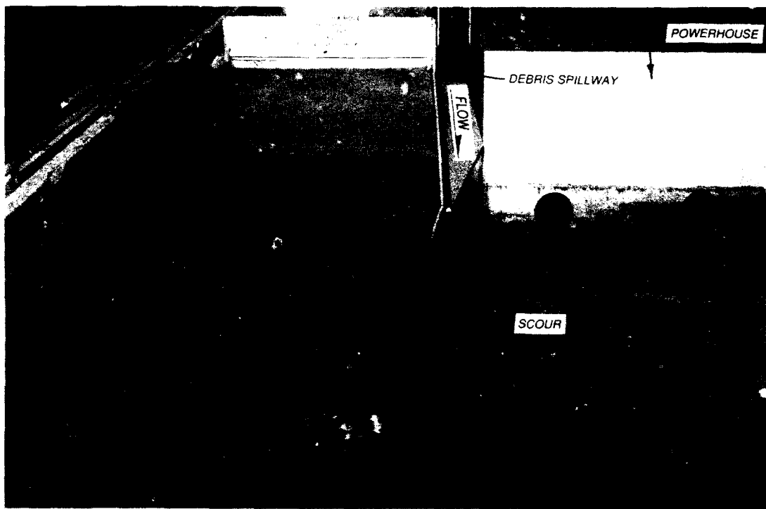
Photo 5. Scour downstream, type 1 design debris spillway; discharge 2,640 cfs, pool el 80.8; tailwater varied from el 66.0 to 32.0
