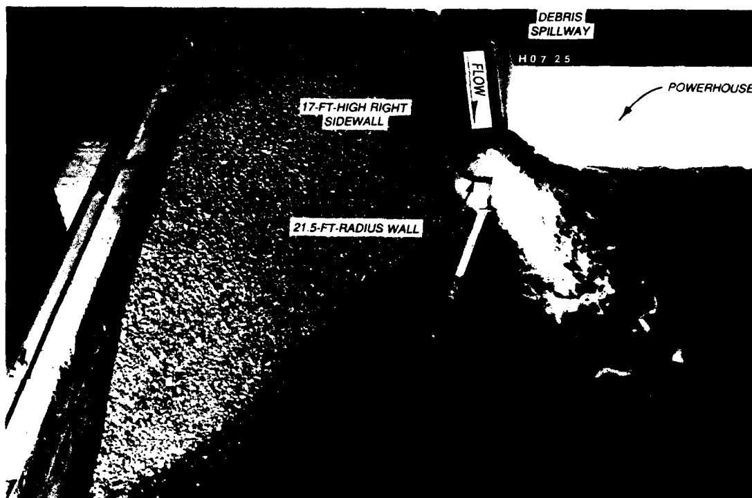
Photo 20. Flow conditions, type 17 design; discharge 2,640 cfs; pool el 80.8; tailwater el 32.0
