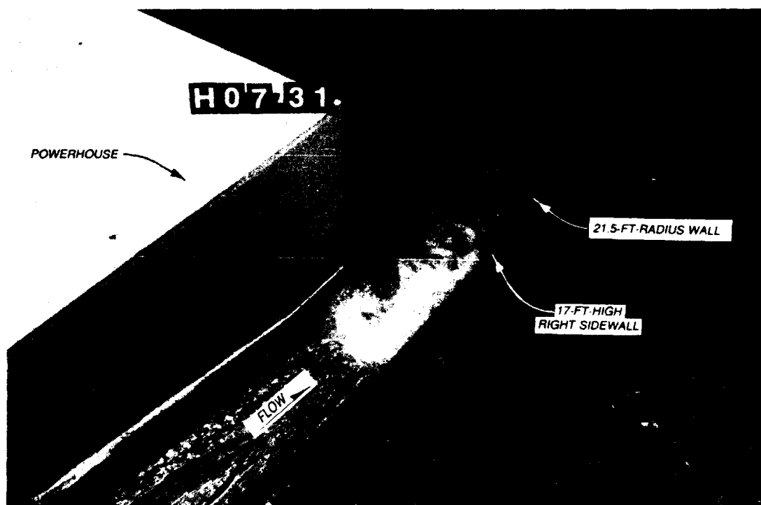
Photo 14. Flow conditions, type 17 design, chute flow; discharge 2,640 cfs; pool el 80.8; tailwater el 50.0
