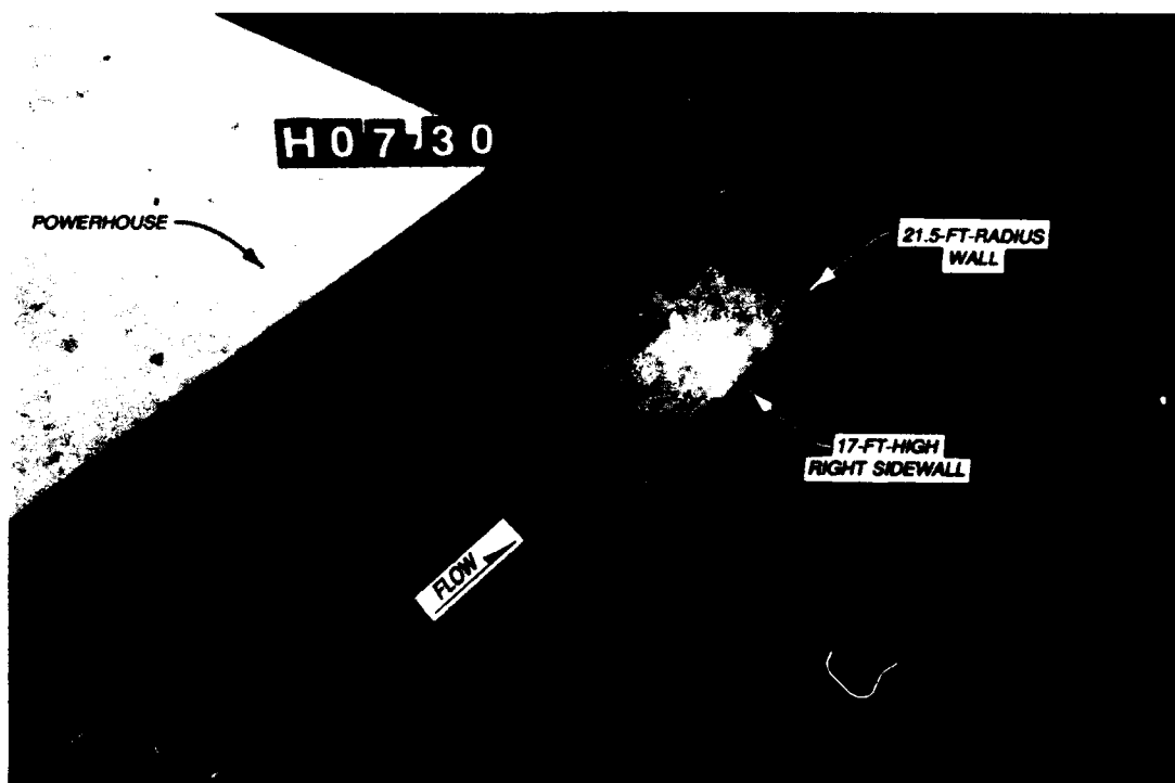
Photo 15. Flow conditions, type 17 design, chute flow; discharge 2,640 cfs; pool el 80.8; tailwater el 40.0
