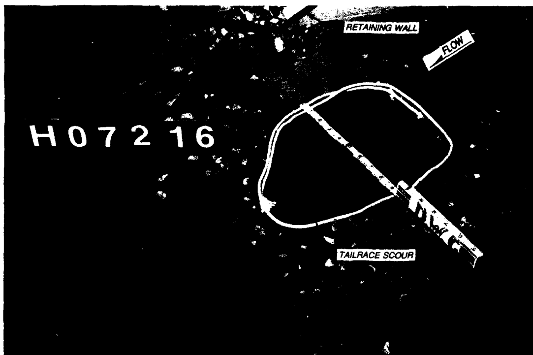
Photo 11. Scour in the tailrace riprap, type 3 design, discharge 2,640 cfs; pool el 80.8; tailwater el 32.0, 2.5 hr
