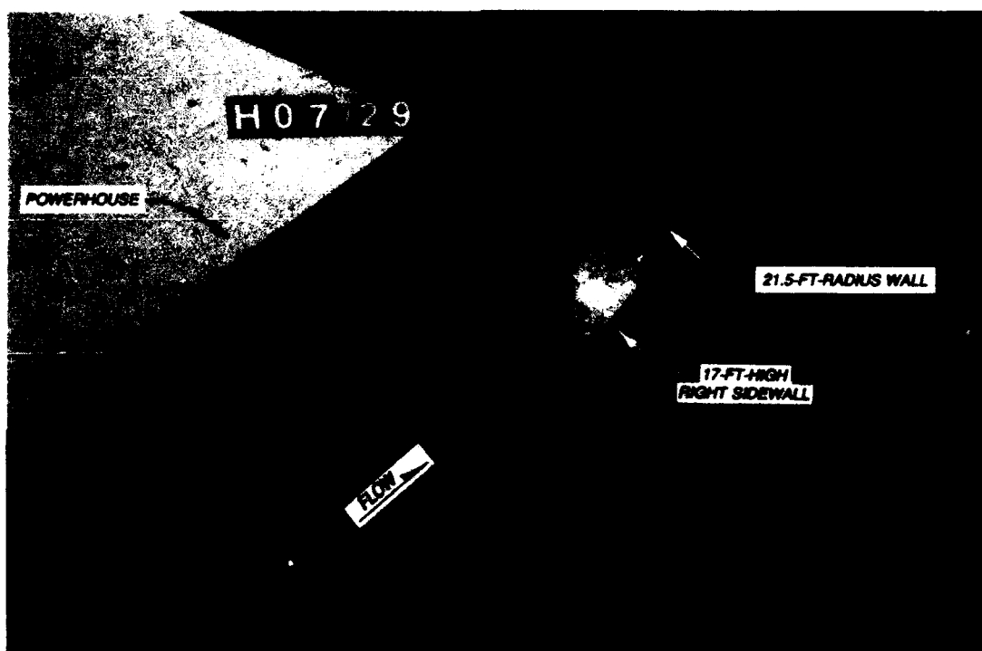
Photo 16. Flow conditions, type 17 design, chute flow; discharge 2,640 cfs; pool el 80.8; tailwater el 32.0
