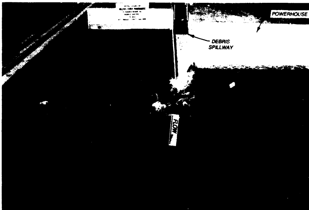
Photo 3. Flow conditions, type 1 design, discharge 2,640 cfs; pool el 80.8; tailwater el 40.0
