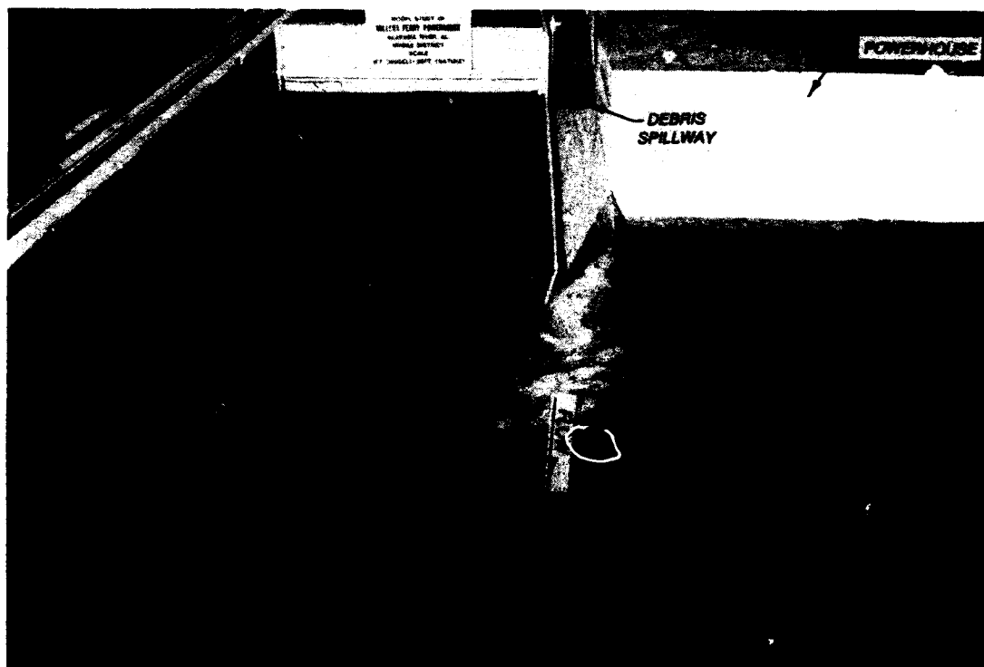
Photo 4. Flow conditions, type 1 design, discharge 2,640 cfs; pool el 80.8; tailwater el 32.0
