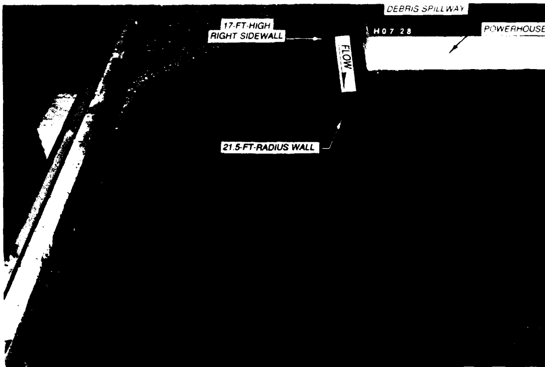
Photo 17. Flow conditions, type 17 design; discharge 2,640 cfs; pool el 80.8; tailwater el 66.0
