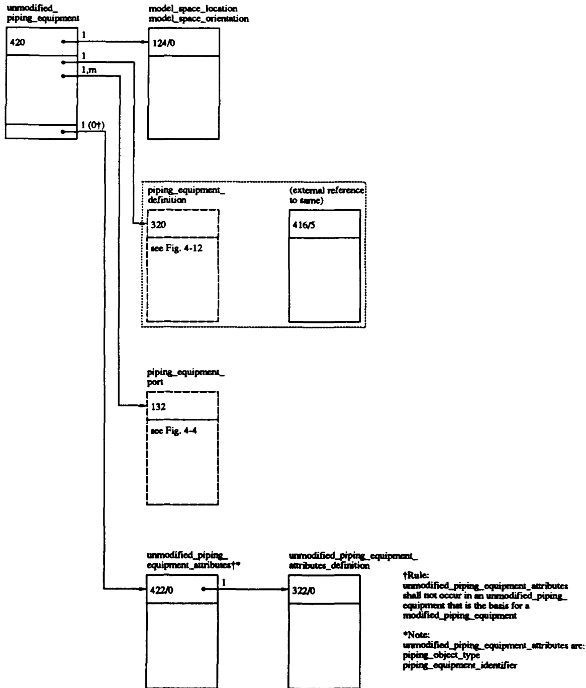
3D Piping AIM Figure 4-10. Unmodified piping equipment
