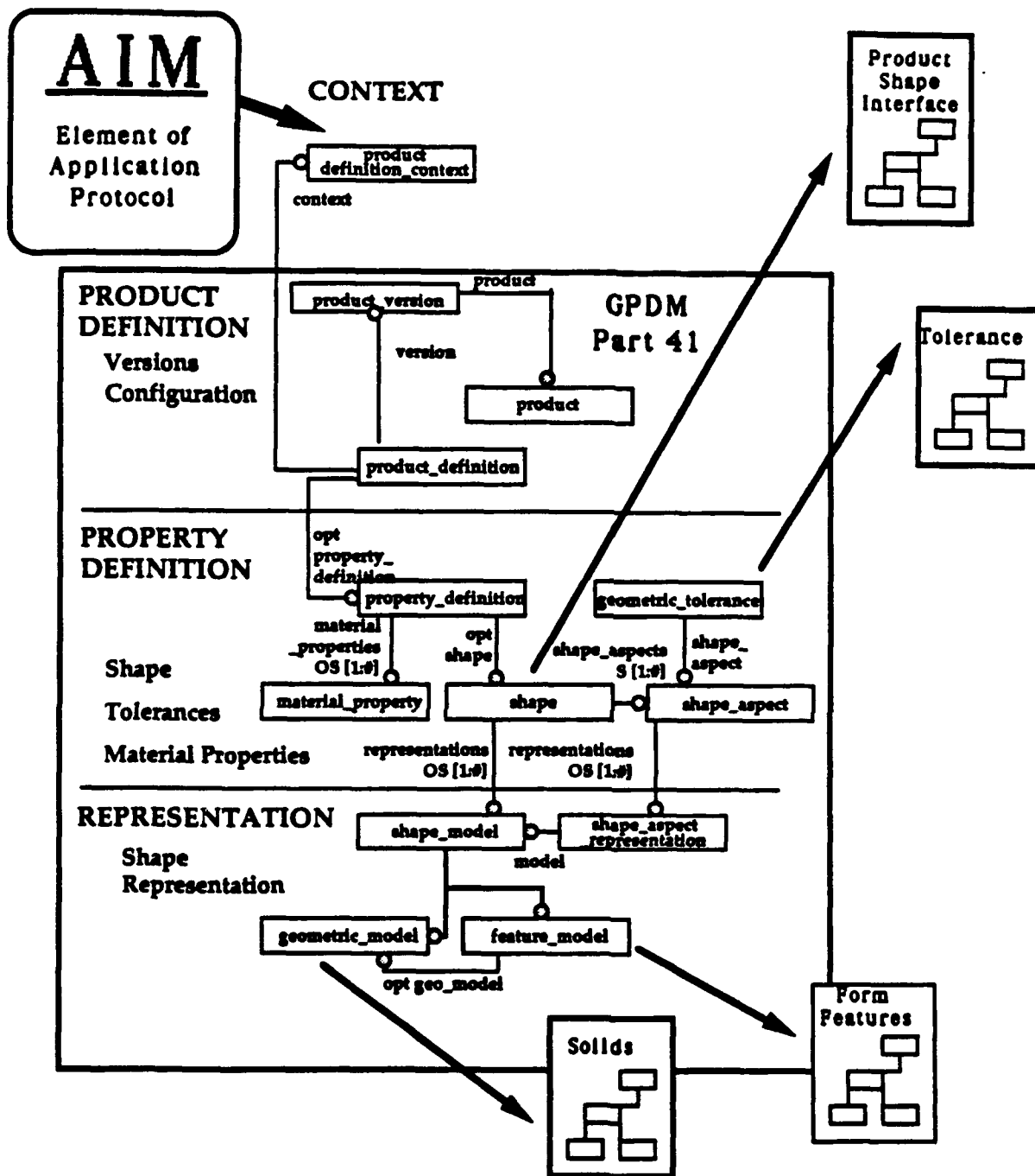
Figure 4. Application Interpreted Model (AIM)
