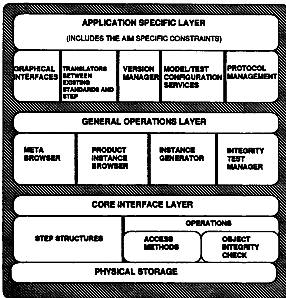
Figure 6. VTS Software Architecture
