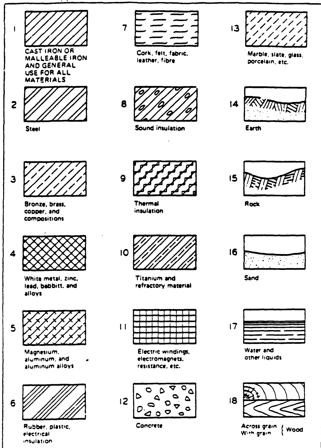
Figure 14. Hatch Styles from Y14.2M
