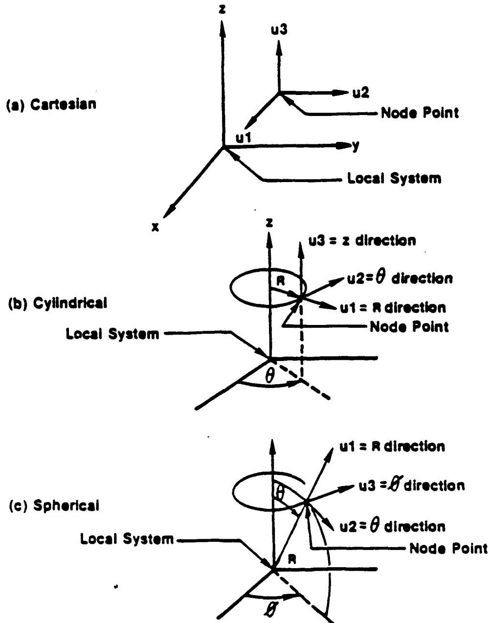
Figure 3-17 Displacement Components
