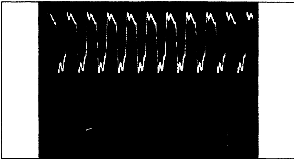
Figure 2.3: Crystal oscillator output. Oscilloscope settings: X = 0.2 \mu sec/Div., Y = 2.0 v/Div. .
