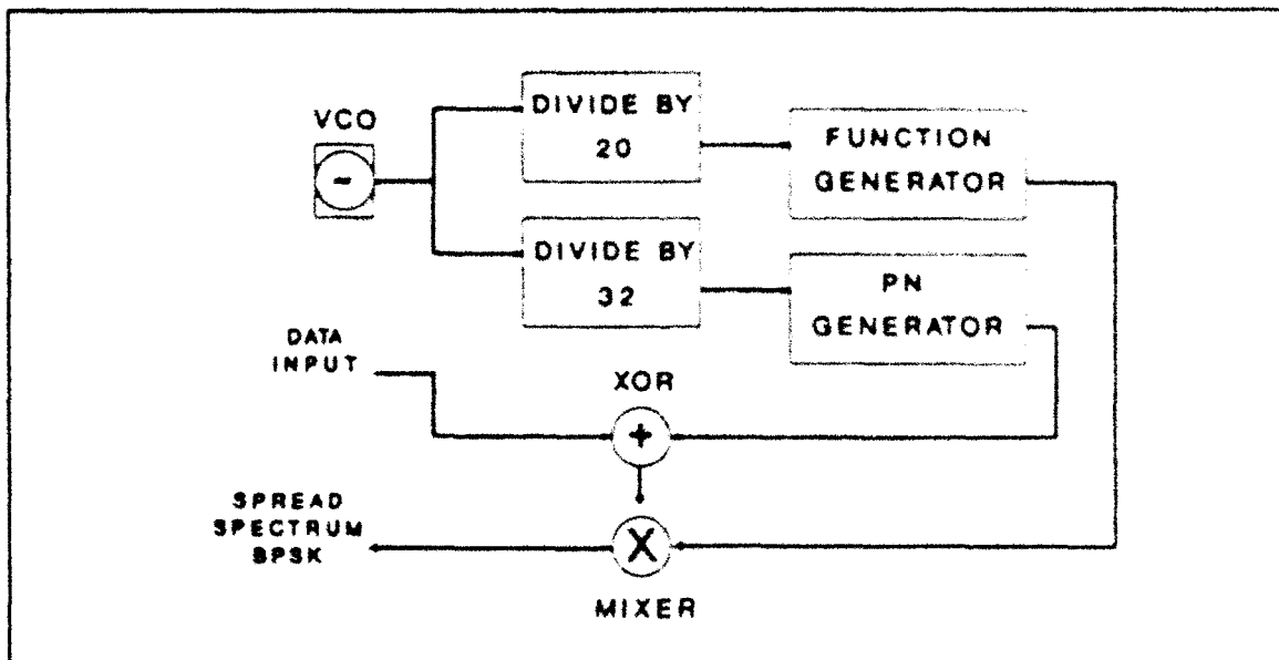
Figure 2.1: Modulator functional block diagram.
