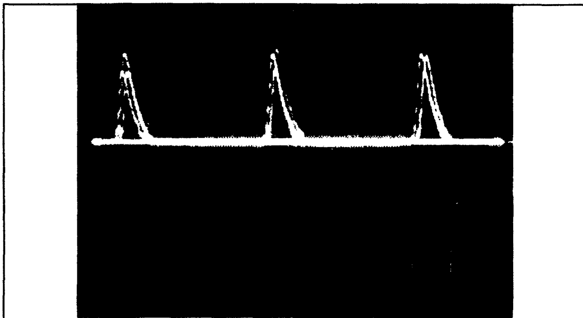
Figure 2.14b: Punctual channel correlation triangle. Oscilloscope settings: X = 0.1 msec/Div., Y = 5 v/Div.
