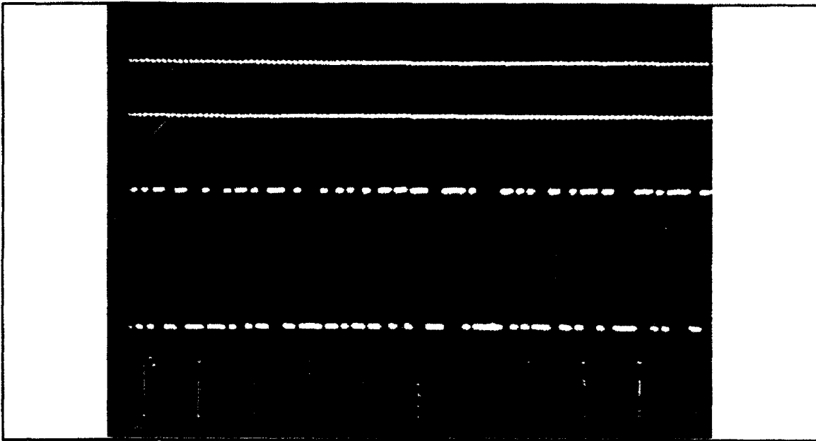
Figure 2.5: Top: PN generator clock (153.6 kHz), 2 v/Div. . Bottom: PN sequence used for spreading, 5 v/Div. .
