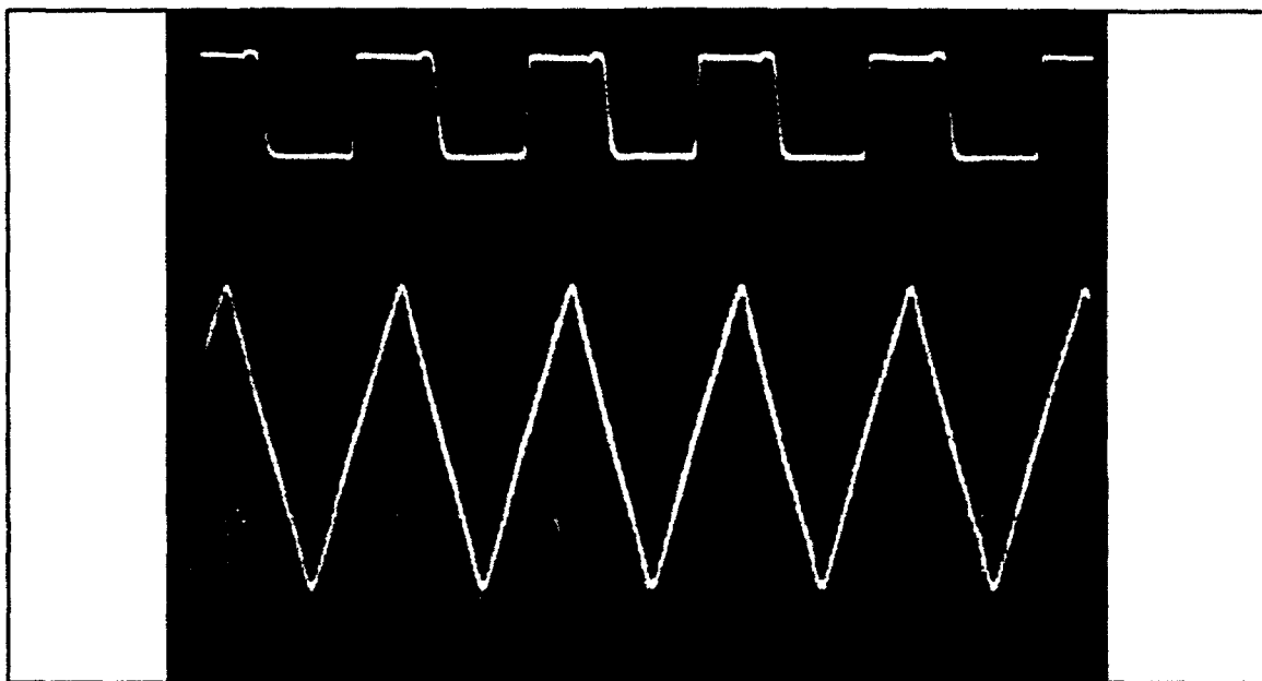
Figure 2.7: Top: 245.7 kHz Square wave; LM311P output. Bottom: Triangle wave output of LM318N integrator. Oscilloscope setting: X = 2 \mu\text{s}/\text{Div.} , Y = 5 v/Div. .
