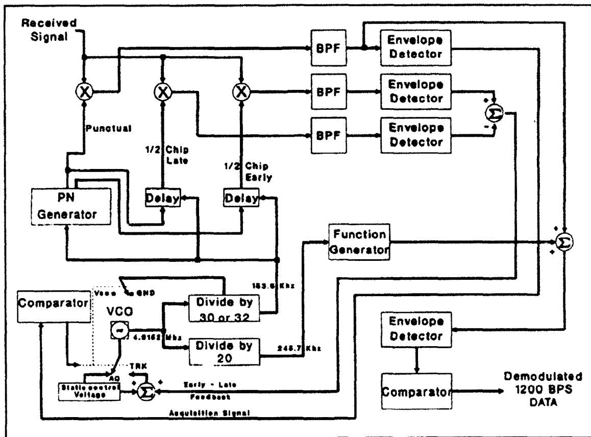
Figure 2.2: Demodulator functional block diagram.
