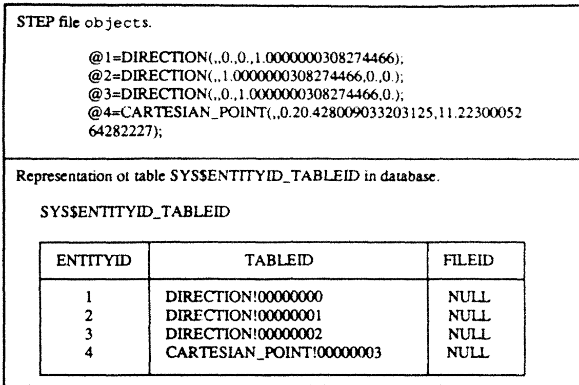
Figure 1: STEP File objects &amp; SYS$ENTITYID_TABLEID Table
