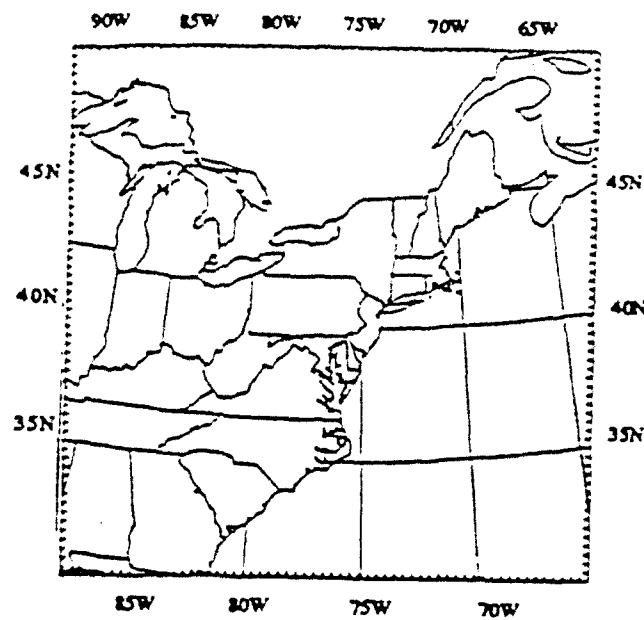
Figure 2: Domain utilized in this work.
