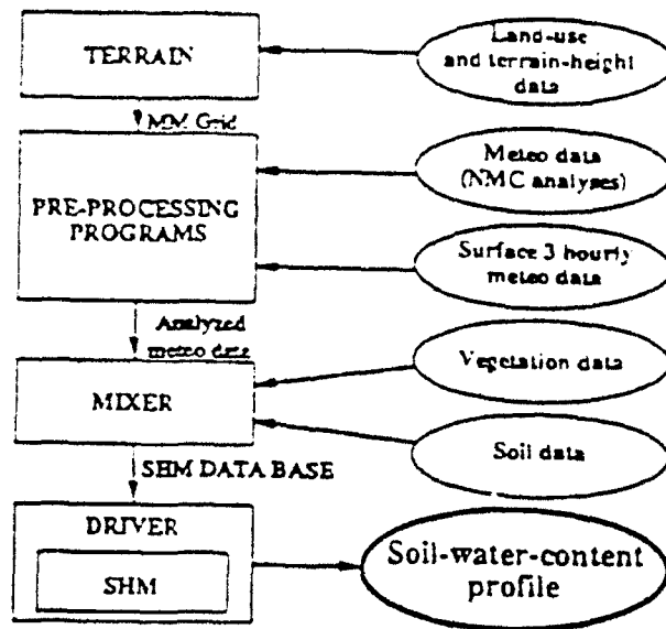
Figure 3: Schematic of the different steps required to obtain the data base for the SHM. MM stands for the Penn State/NCAR Mesoscale Model.
