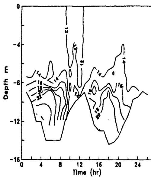
Anchor 2 Salinity
