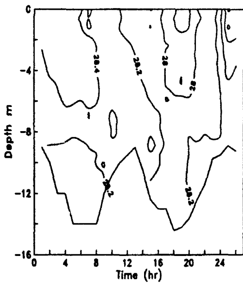
Anchor 2 Temperature
