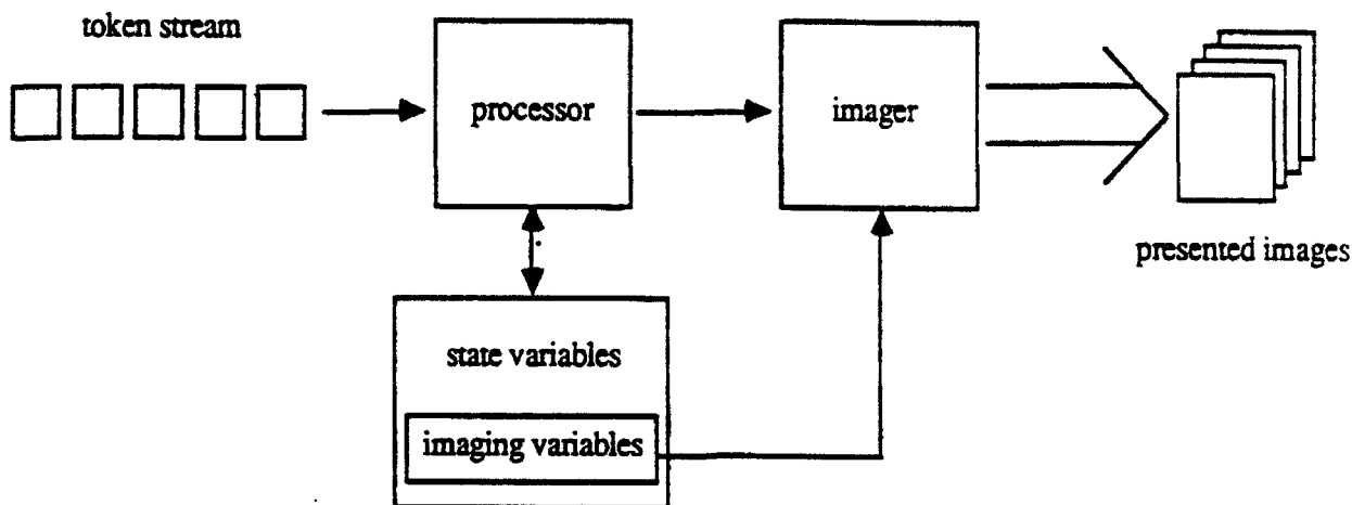
Figure 2. Basic Operational Model for Static PDLs
