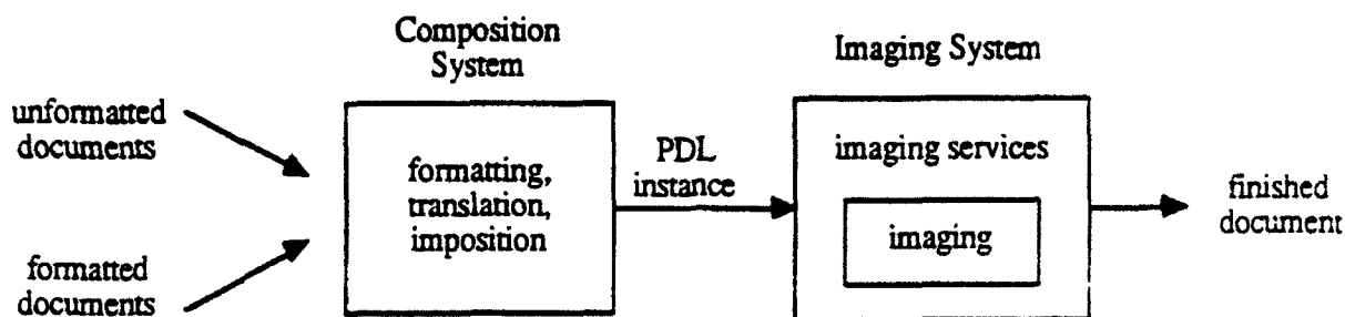
Figure 1. A simplified Model for Document Processing
