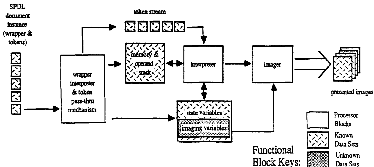
Figure 2. An SPDL Rendering System
