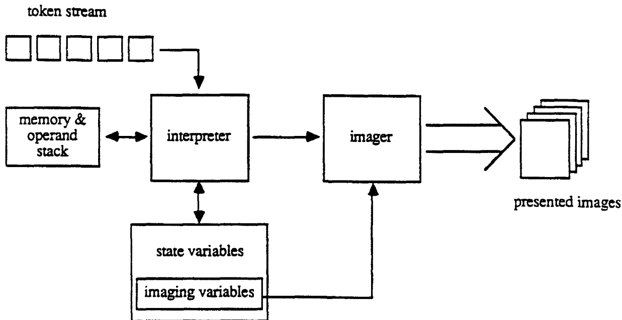
Figure 3. Basic Operational Model for Programmable PDLs
