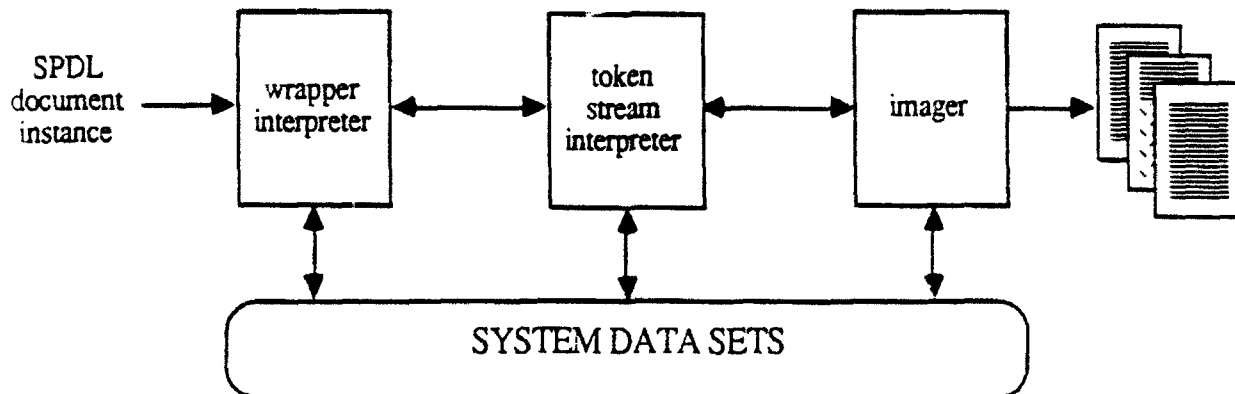
Figure 1. Overview Of An SPDL Imaging System
