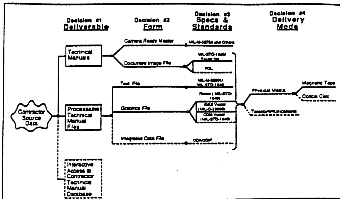
Figure 1. Decision Template
