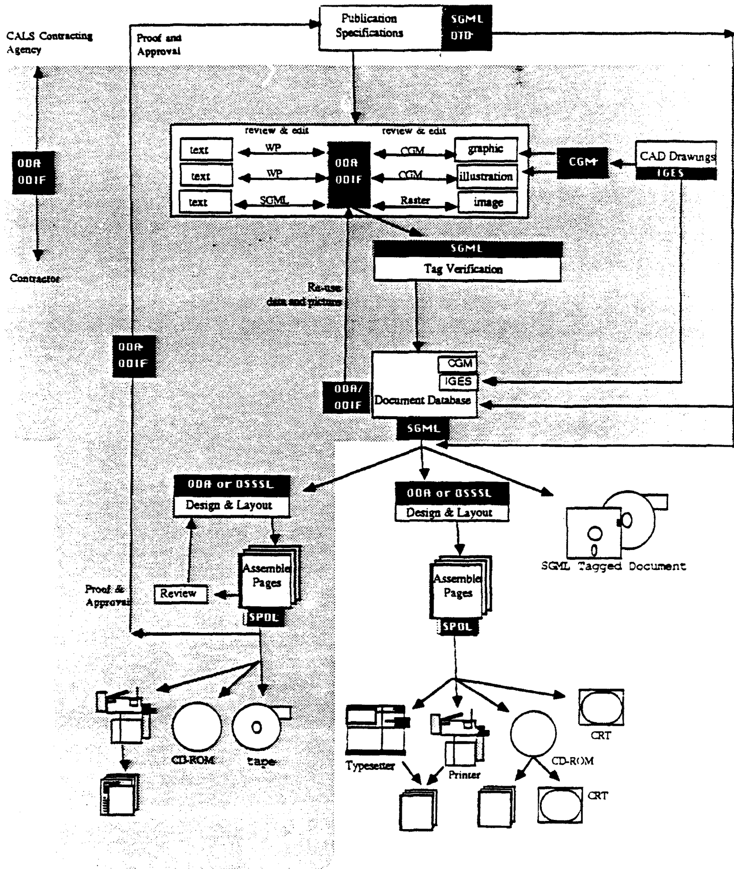
Figure 3: Publishing Model and Standards
