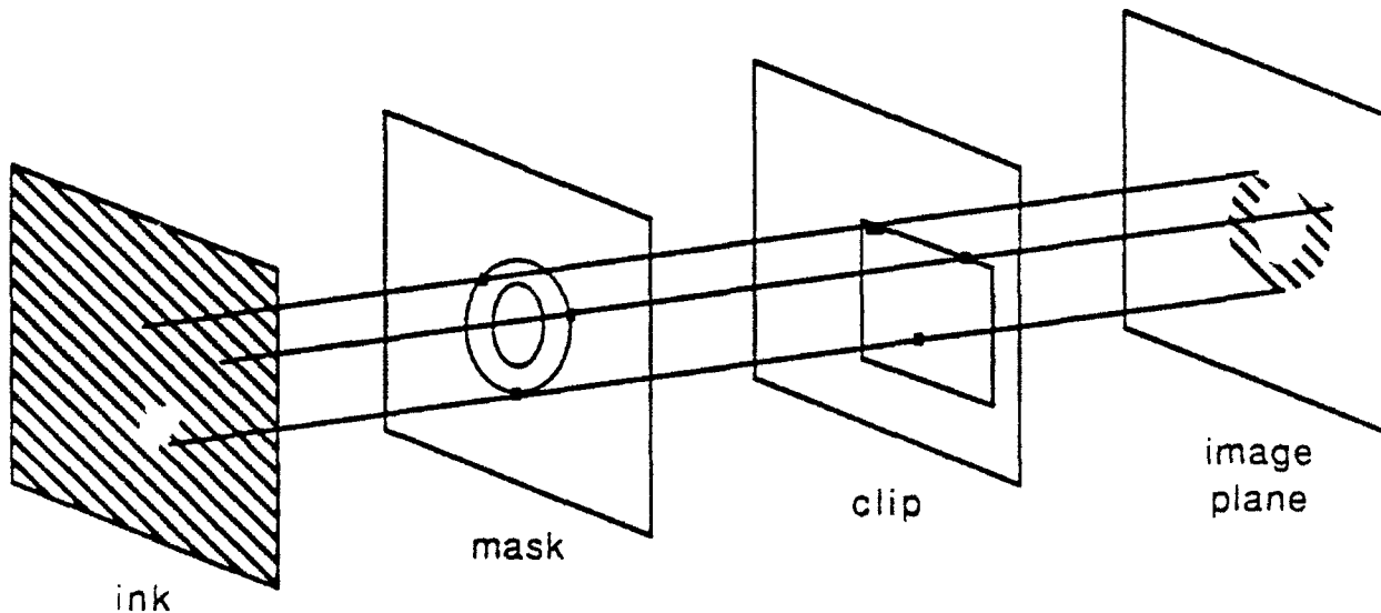
Figure 5. A richer imaging model for a device independent colour PDL
