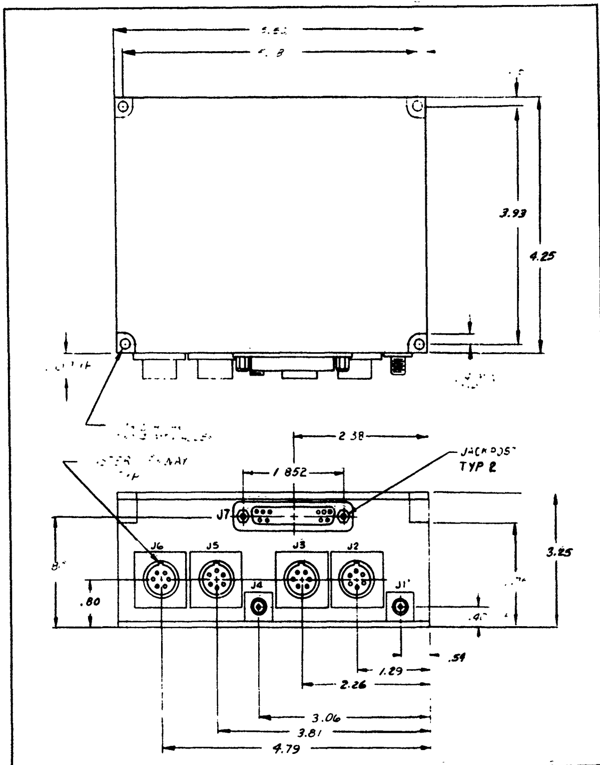
Figure 4-19. Outline drawing of LC Model CDR-555 Flight Termination Receiver.
