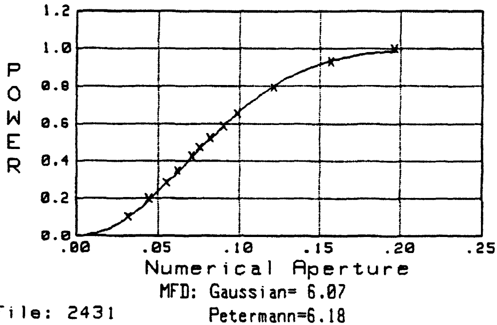
Figure 8 Coupler Fiber Numerical Aperture
