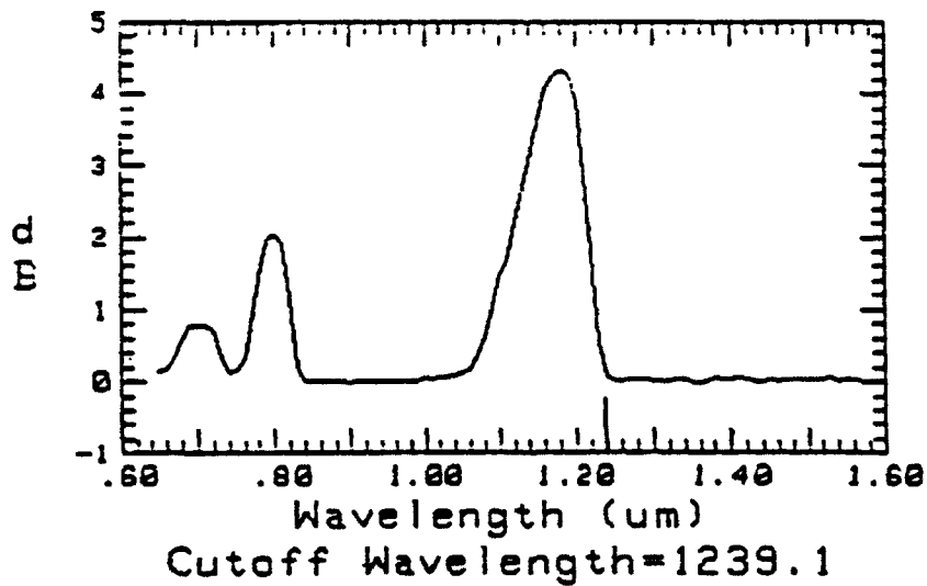
Figure 2 Fiber Cutoff Plot
