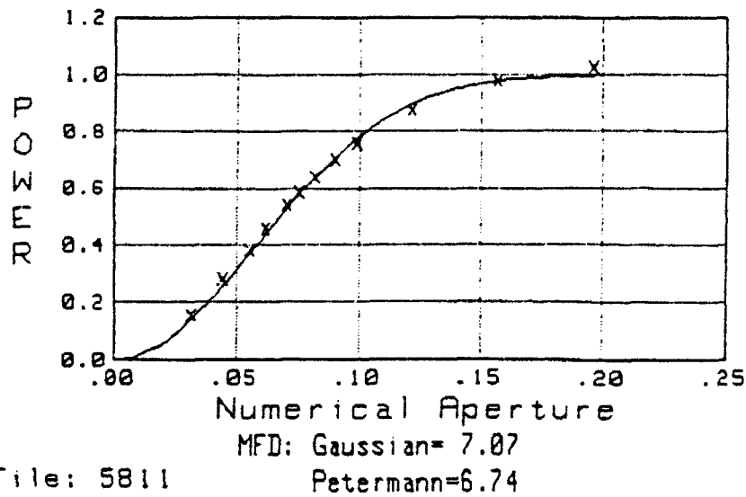
Figure 9 Mode Field Diameter (60 \mu m Diameter)
