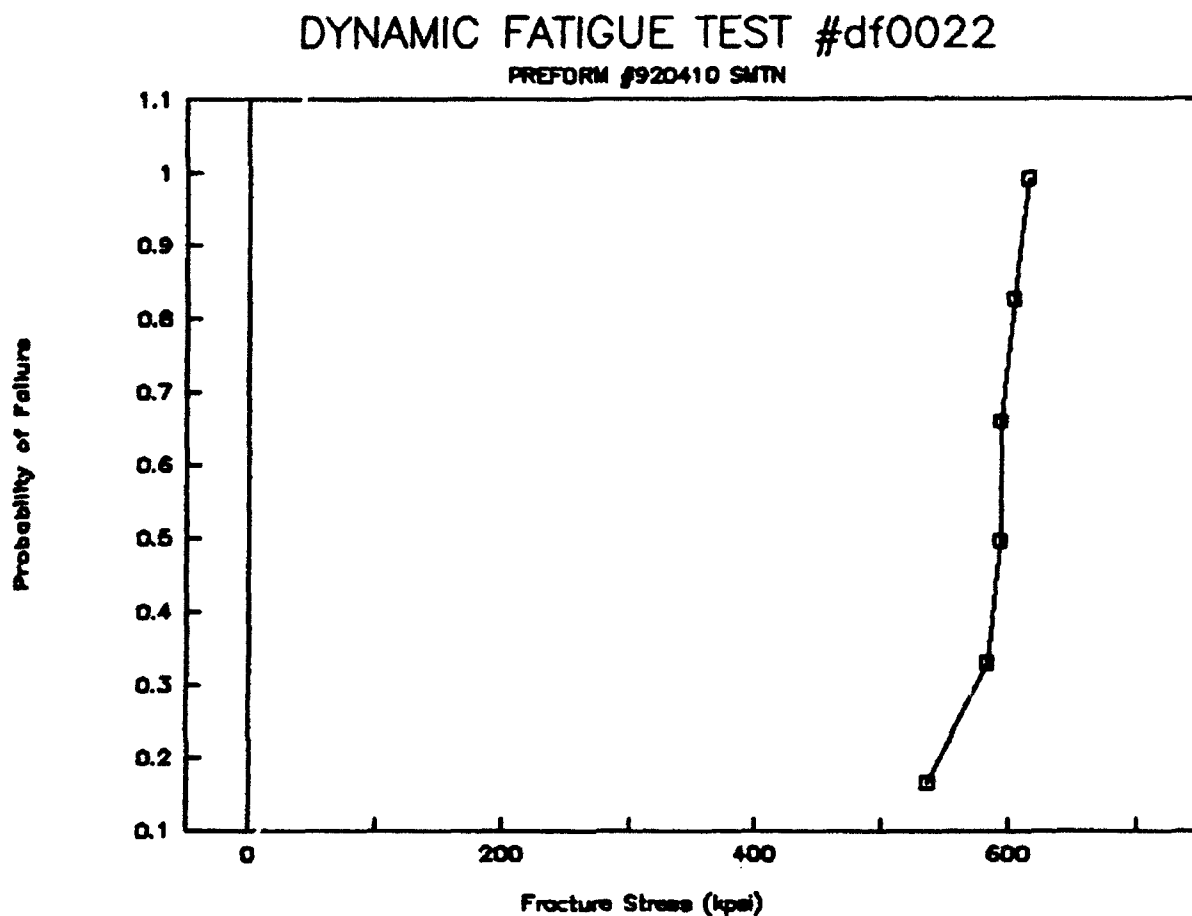
Figure 4 Fiber Strength
