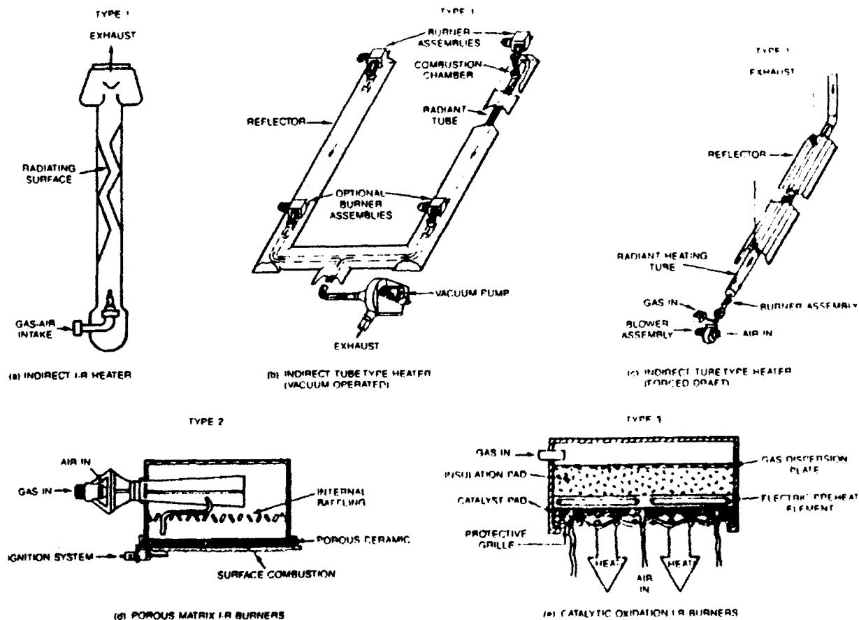
Figure 1. Types of Gas-Fired Heaters. (Reprinted with permission from the American Society of Heating, Refrigerating and Air-Conditioning Engineers, from the 1988 ASHRAE Handbook - Equipment.)
