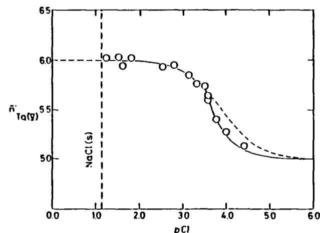
Figure 1. Average experimental coordination number (with precipitate included) ( n'_{\text{Ta(V)}} ) for Ta(V) in NaCl-AlCl 3 at 175 °C as a function of pCl. The formal concentrations (in the pCl range where no precipitate was present) were 0.23-0.30 F. Calculated values of n' (for the reaction \text{TaCl}_5 \leftrightarrow \text{TaCl}_3 + \text{Cl} ) are indicated by a full curve. The dashed curve shows for a hypothetical extrapolation what would happen if no precipitation occurred. The vertical dashed line shows the limiting pCl, due to saturation with NaCl.
