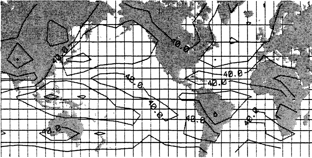
(a) CLIMA-TV contour map of mean total cloud amount for January.
