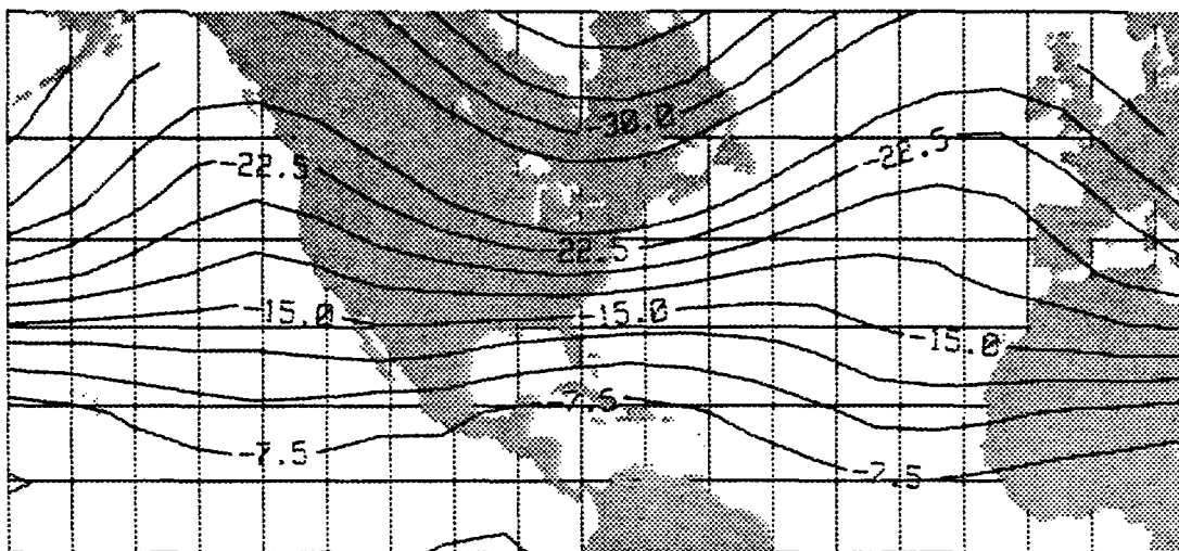
(a) CLIMA-TV contour map of mean 500 mb temperature for January.
