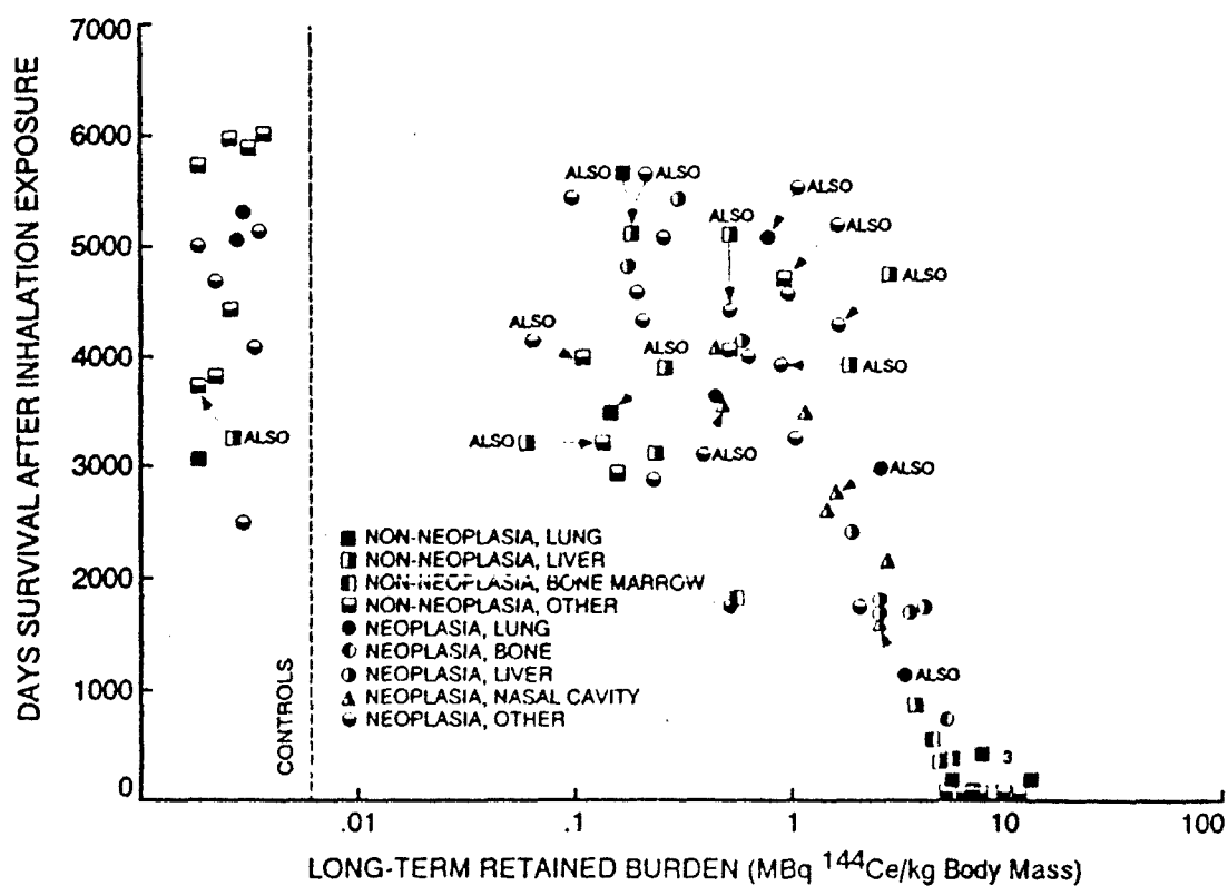
Figure 25. Relationship between long-term retained burden and survival time for Beagle dogs that inhaled ^{144}\text{CeCl}_3 .
