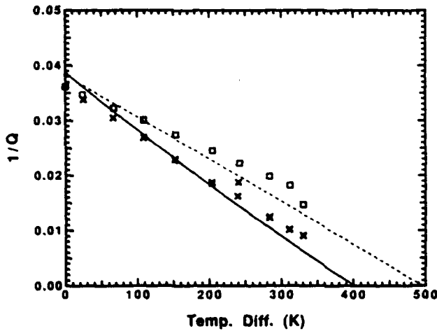
FIG. 7. Graph of 1/Q versus the temperature difference across the prime mover stack for the second and third longitudinal modes. The \times 's and solid line correspond to the second mode, while the open squares and dashed line correspond to the third. The prime mover is filled with helium at a mean pressure of 170 kPa.
