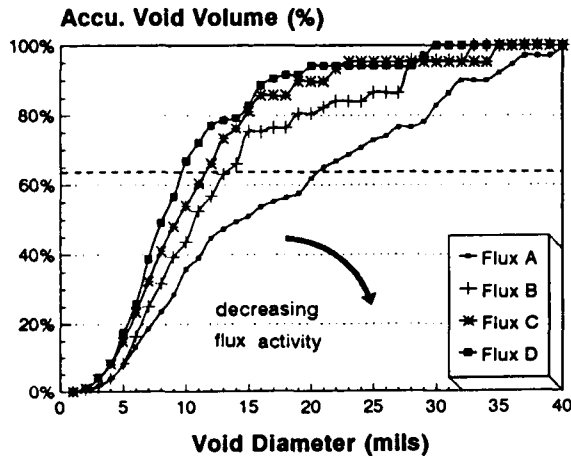
Figure 16 Effect of flux activity on void size distribution
