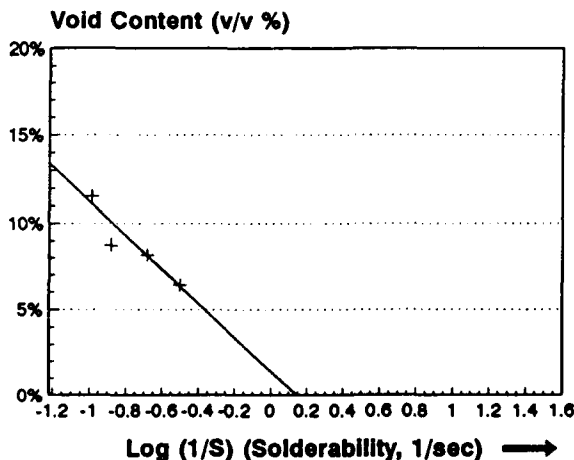
Figure 10 Effect of solderability on voiding
