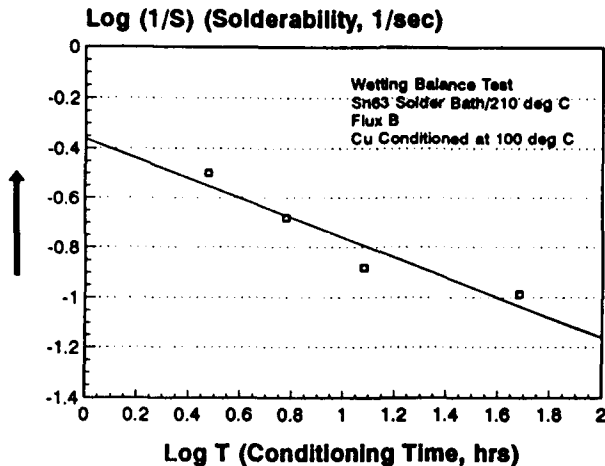
Figure 9 Relation between conditioning time and solderability
