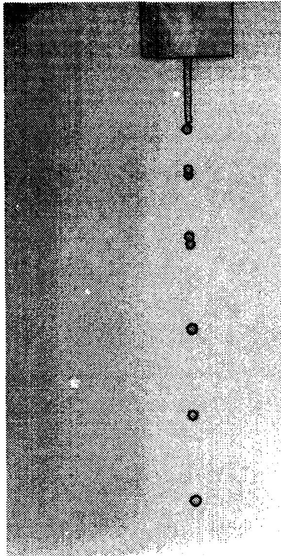
FIGURE 4. Droplet Generation from the Orifice.
