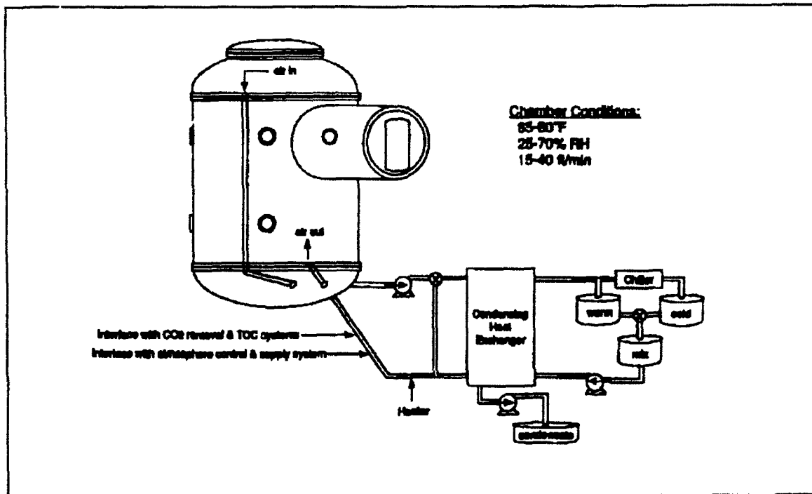
Figure 3.2 Temperature and Humidity Control Subsystem
