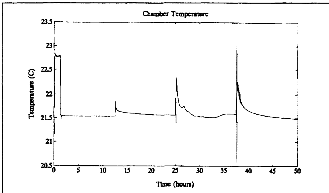
Figure 5.22 Temperature Closed Loop Response to Disturbance
