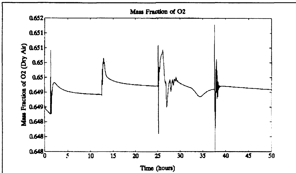
Figure 5.21 Oxygen Mass Fraction Disturbance Response
