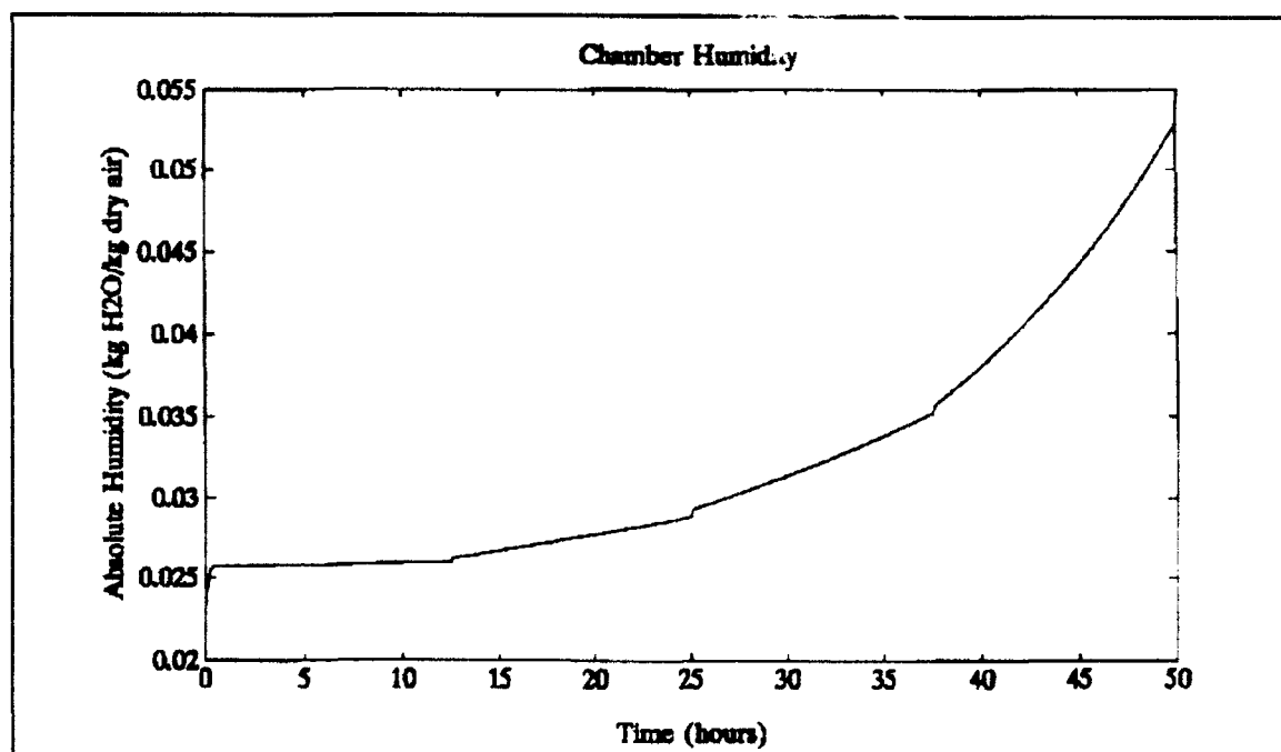
Figure 5.19 Absolute Humidity Open Loop Response
