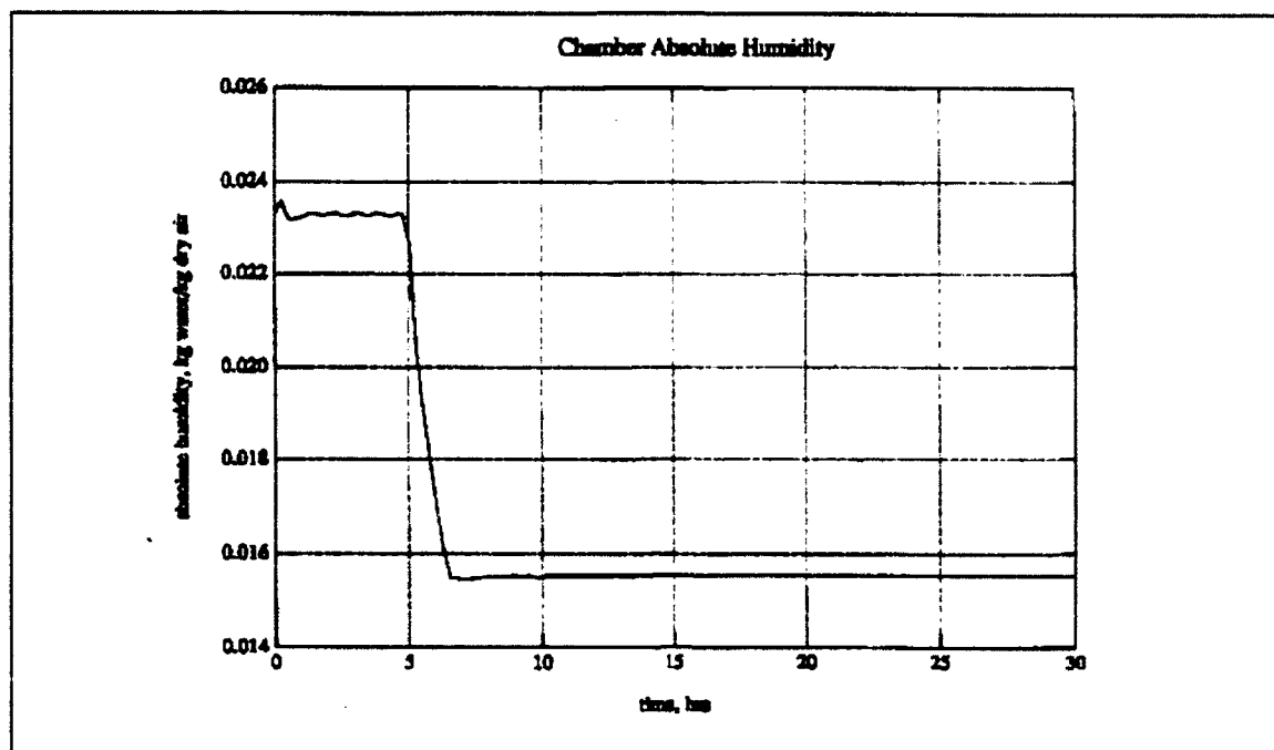
Figure 5.12 Absolute Humidity Transient Response
