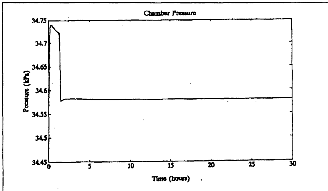
Figure 5.1 Pressure Steady State Response at 34.464 kPa
