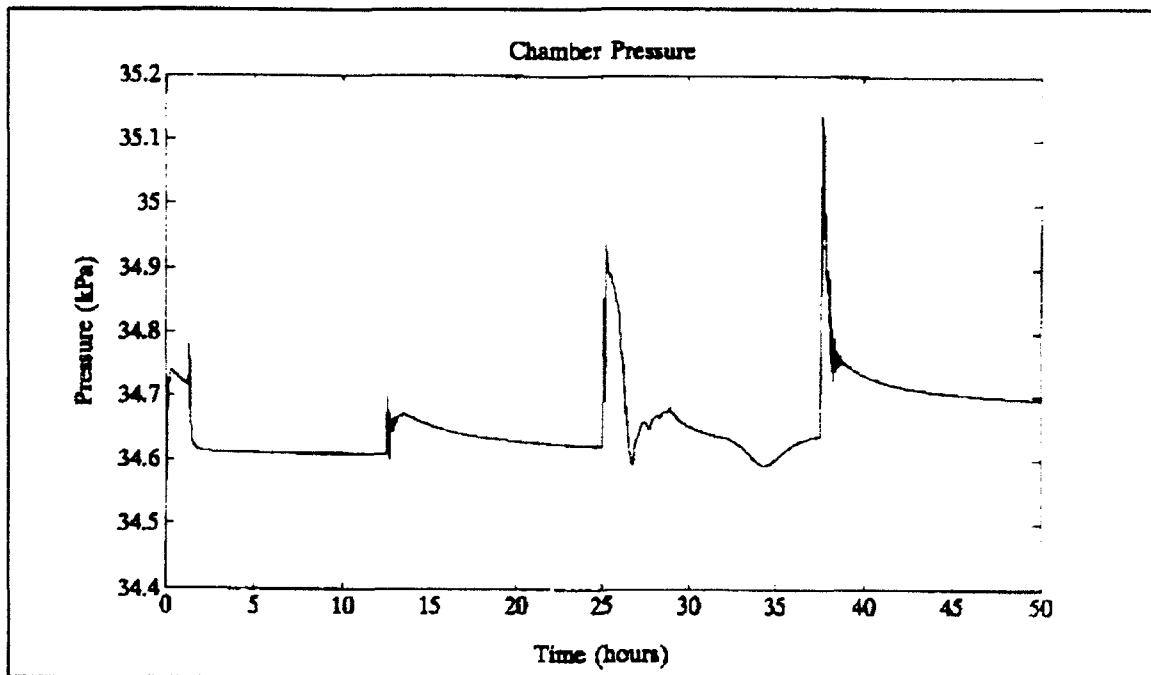
Figure 5.20 Pressure Closed Loop Disturbance Response
