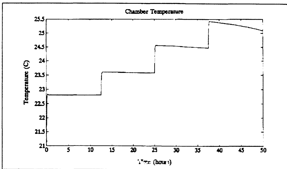
Figure 5.18 Temperature Open Loop Response
