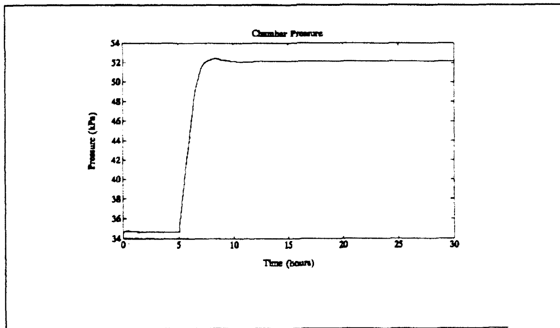
Figure 5.5 Pressure Transient Response
