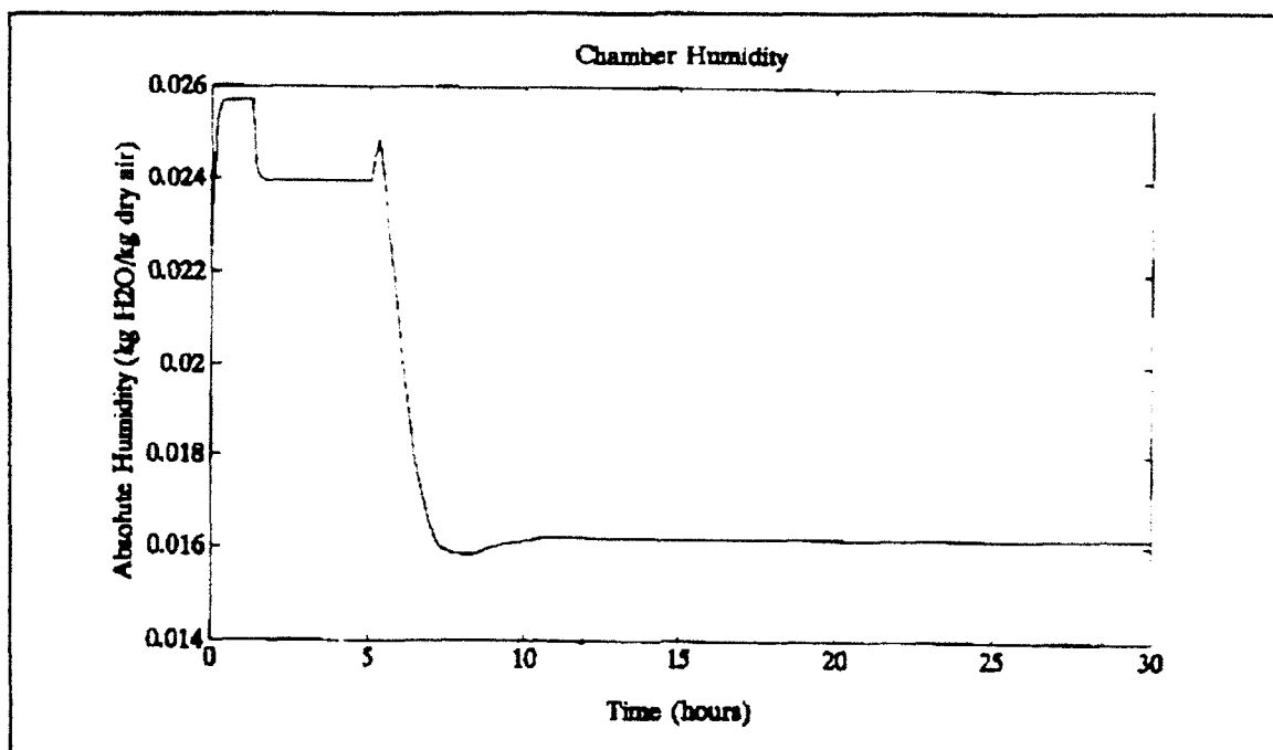
Figure 5.8 Absolute Humidity Transient Response
