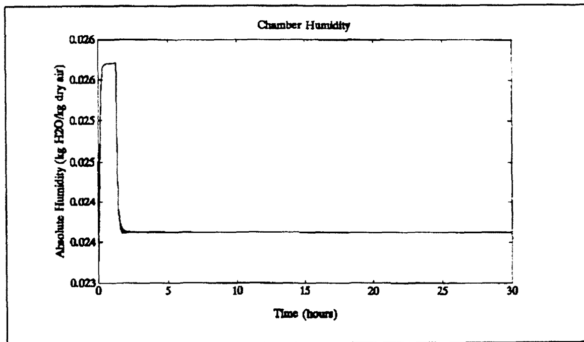
Figure 5.4 Absolute Humidity Steady State Response
