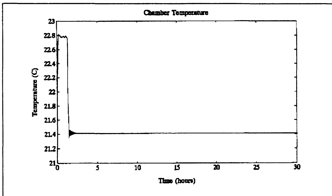
Figure 5.3 Temperature Steady State Response
