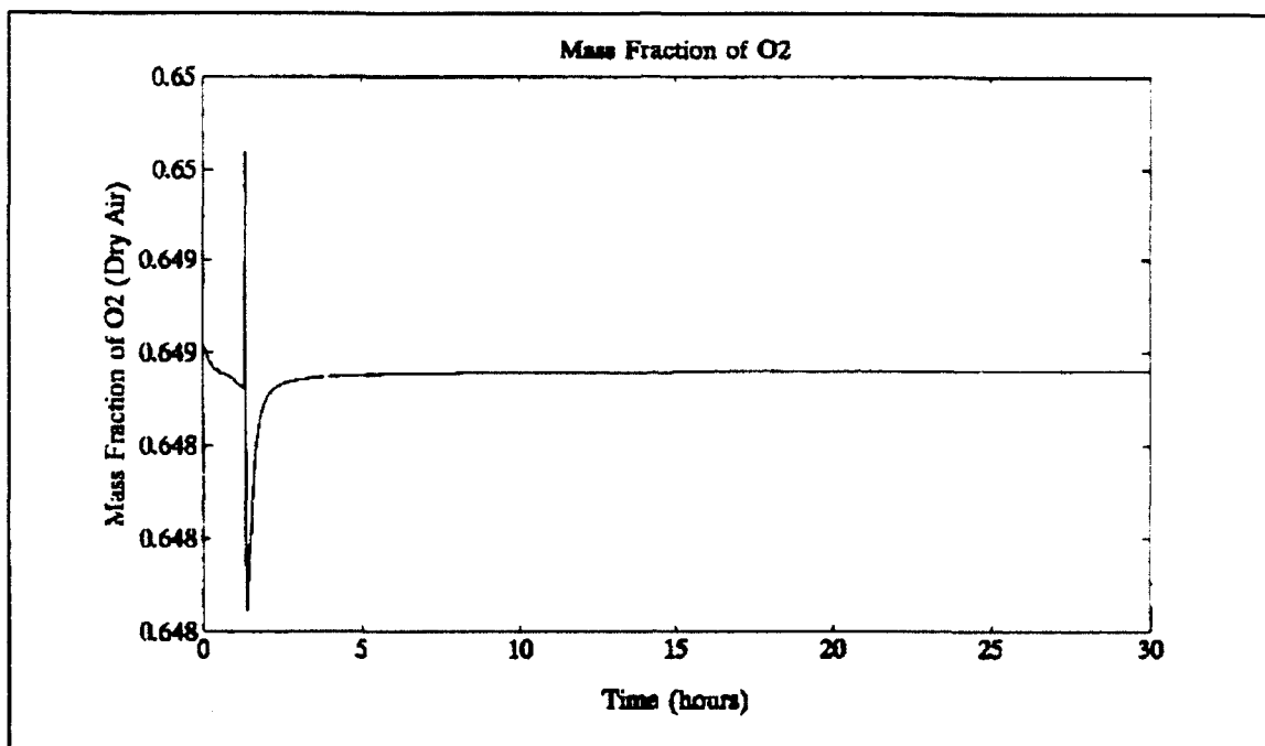
Figure 5.2 Oxygen Mass Fraction Steady State Response
