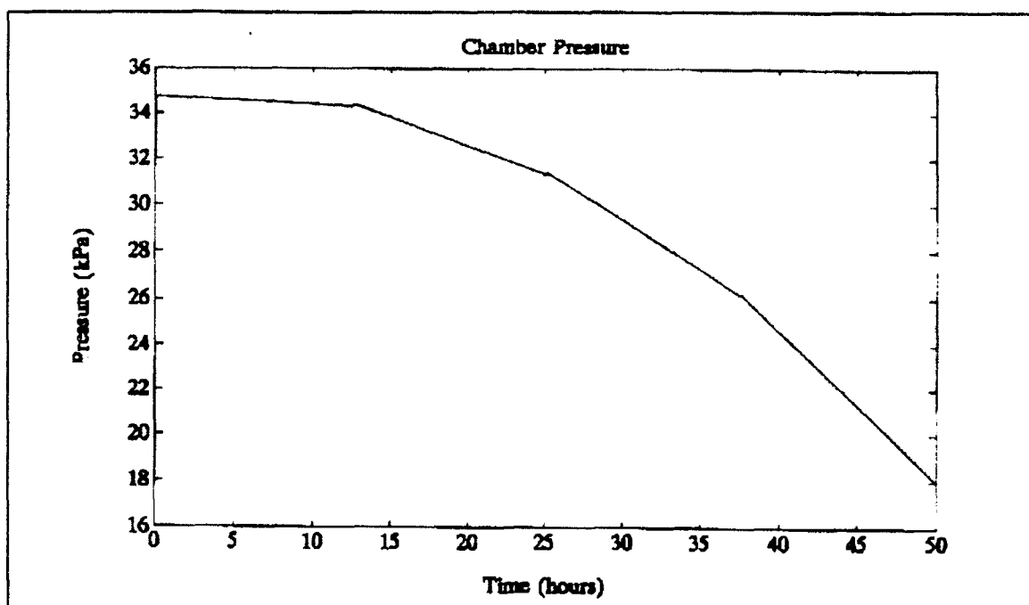
Figure 5.16 Pressure Open Loop Response
