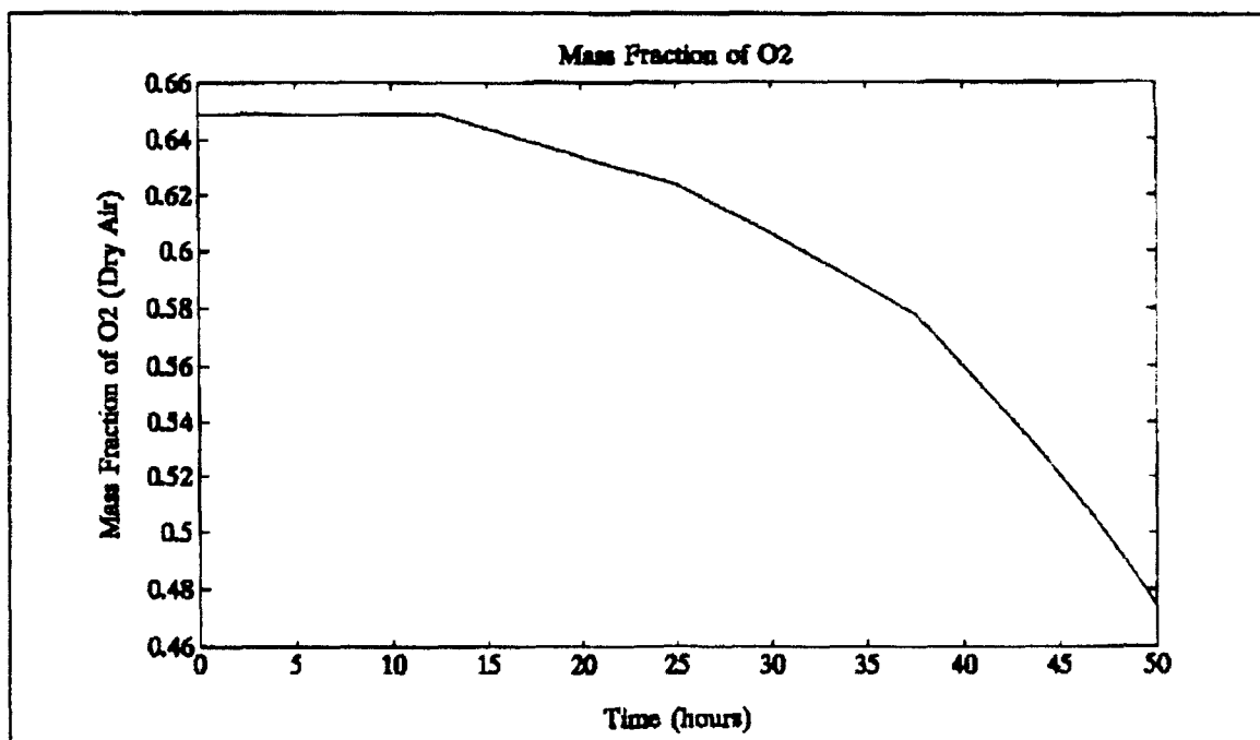
Figure 5.17 Oxygen Mass Fraction Open Loop Response
