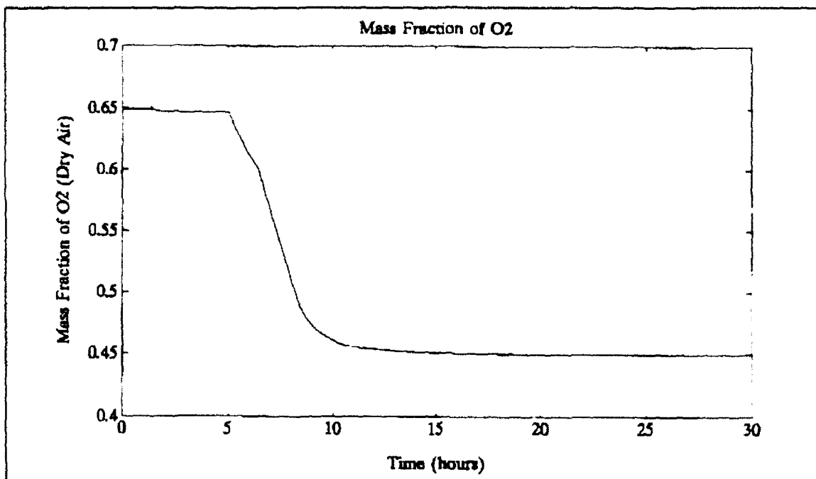
Figure 5.6 Oxygen Mass Fraction Transient Response
