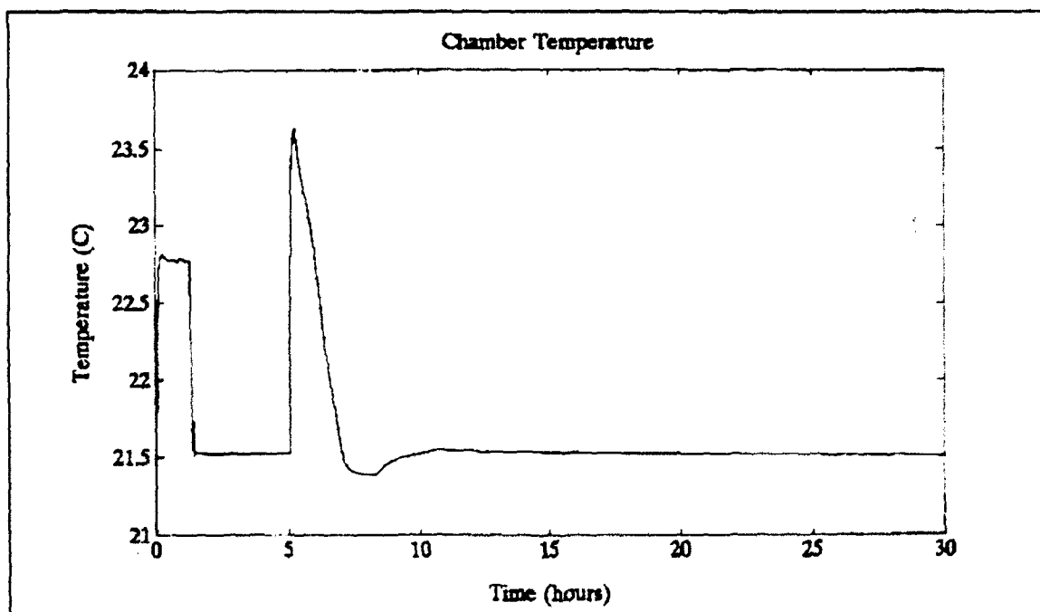
Figure 5.7 Temperature Transient Response
