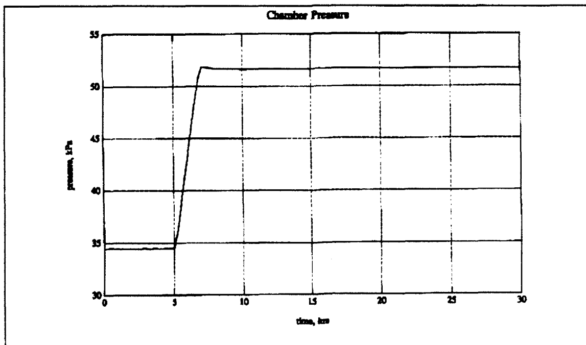
Figure 5.9 Pressure Transient Response
