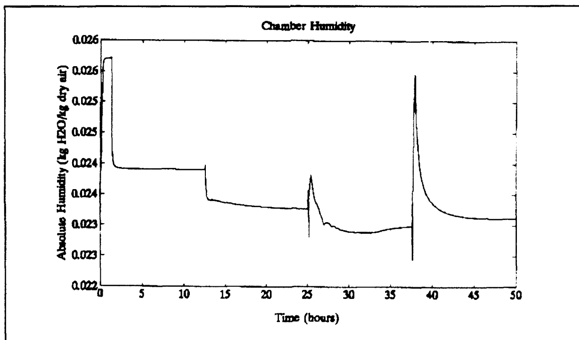
Figure 5.23 Absolute Humidity Closed Loop Response to Disturbance
