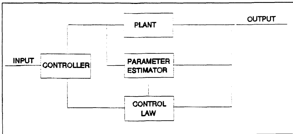
Figure 4.1. Indirect Adaptive Control
