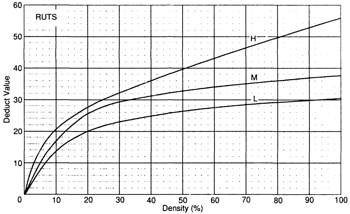
Figure D-6. Distress 86—ruts deduct values.
