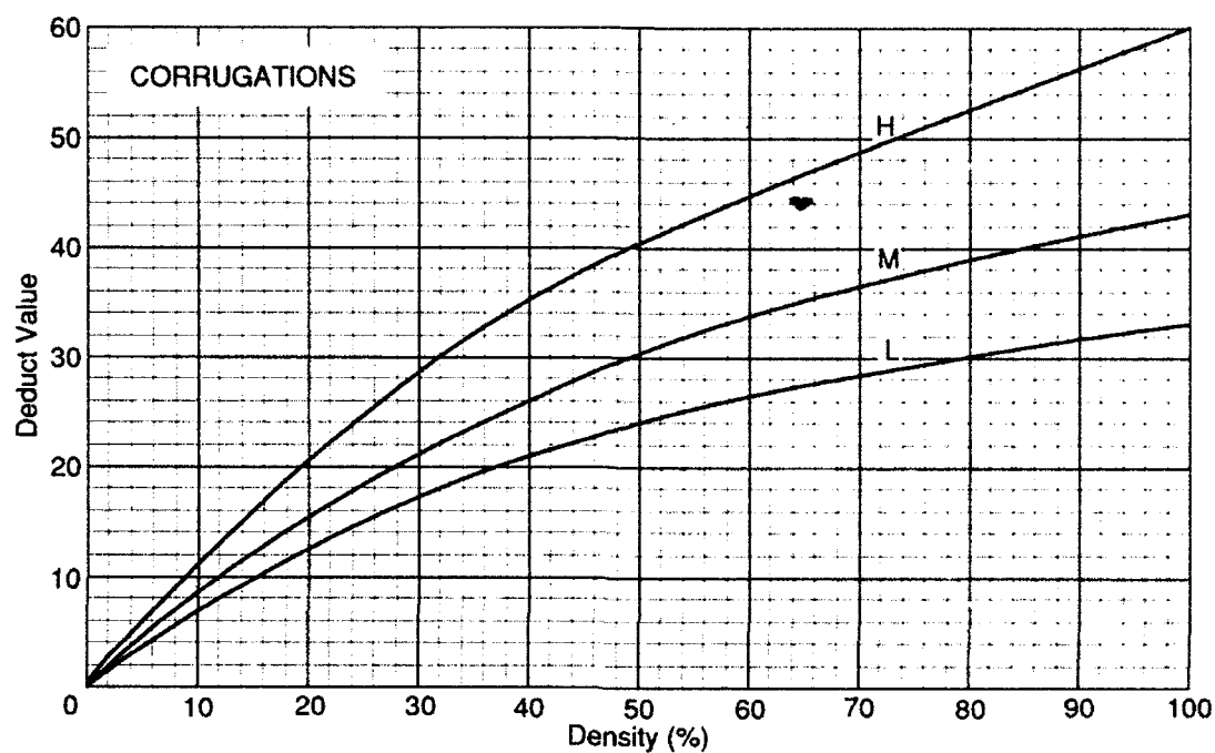
Figure D-3. Distress 83—corrugations deduct values.
