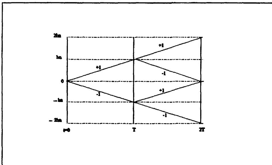
Figure 15 Phase Trellis of Binary CPFSK
