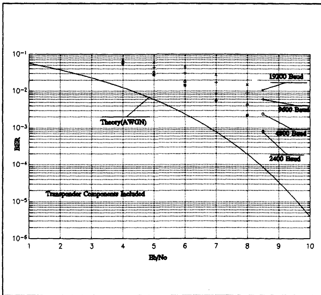
Figure 25 MSK Performance in AWGN Satellite Channel
