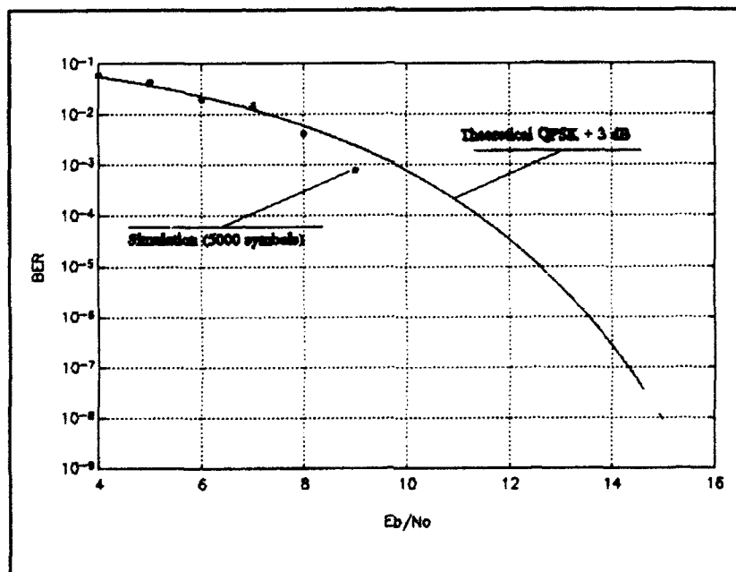
Figure 20 DQPSK Simulation in AWGN
