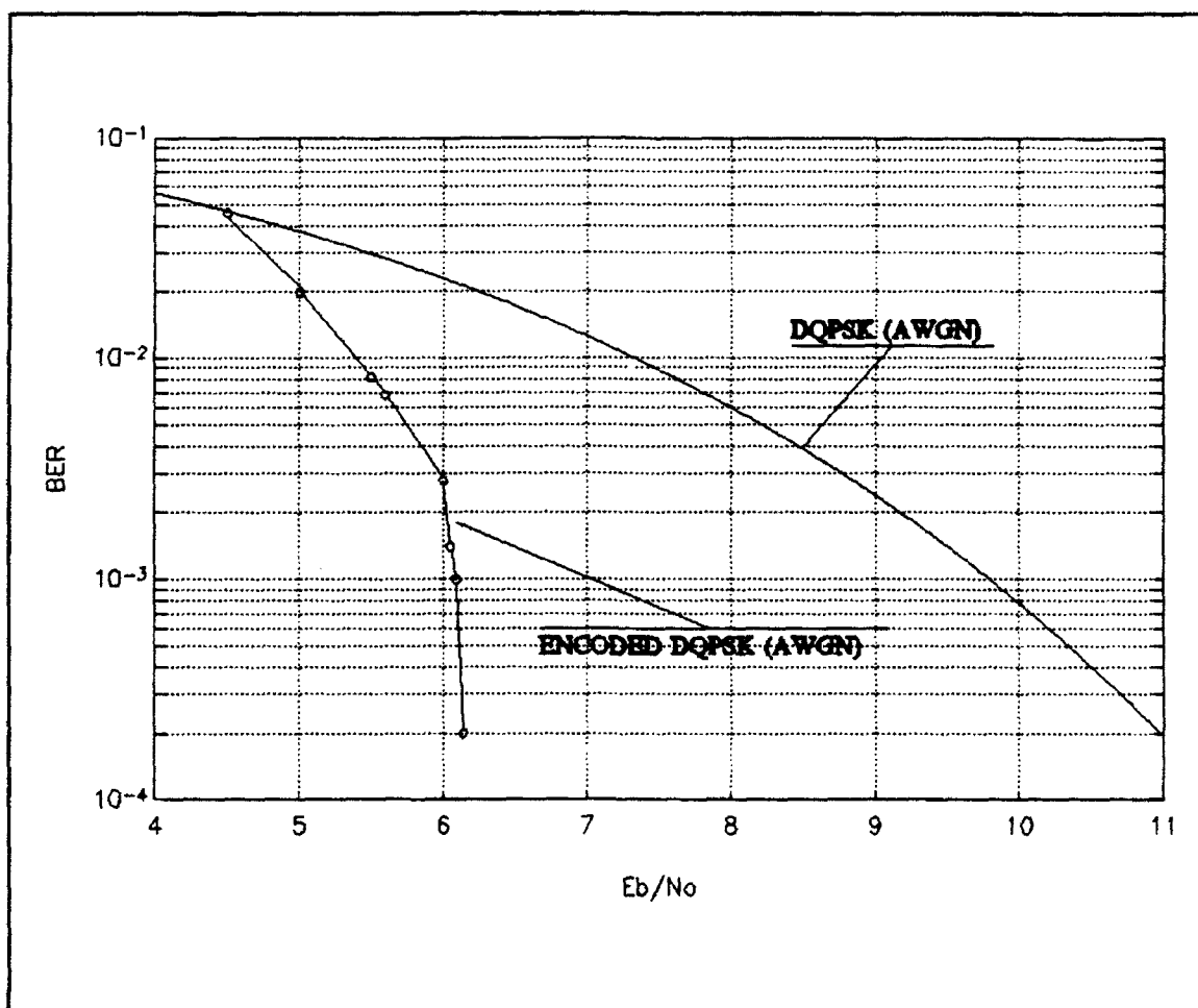
Figure 22 Rate 1/2 Encoded DQPSK in AWGN Satellite Channel
