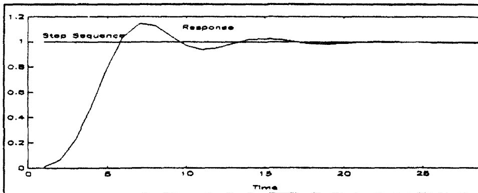
Figure 10 Step Response of Postlimiter Filter
