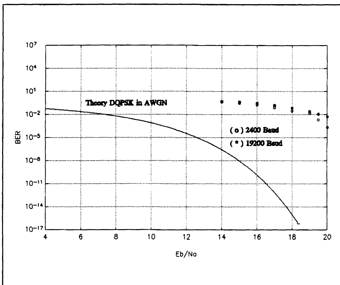
Figure 24 Performance of Rate 1/2 Convolutionally Encoded DQPSK in Fading Satellite Channel
