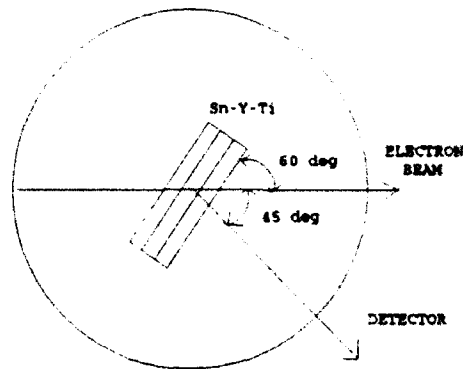
Figure 21. Sandwich foil configuration in the target chamber used in calculating beam intensity.
