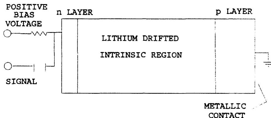
Figure 5. Configuration of p-i-n junction [Ref. 5].
