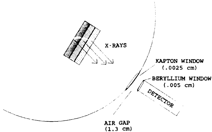
Figure 20. Target ladder configuration and attenuating materials.
