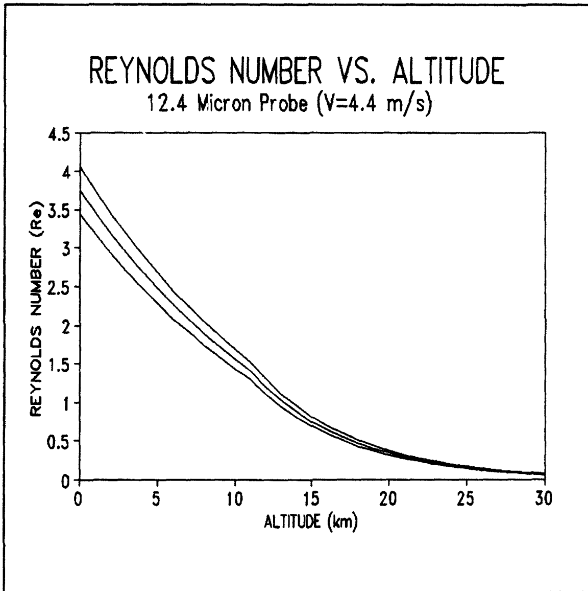
Figure 18: Reynolds Number vs. Altitude for NPS 12.4 \pm 1.0 \mu\text{m} Chromel-Constantan Thermocouple Probe.
