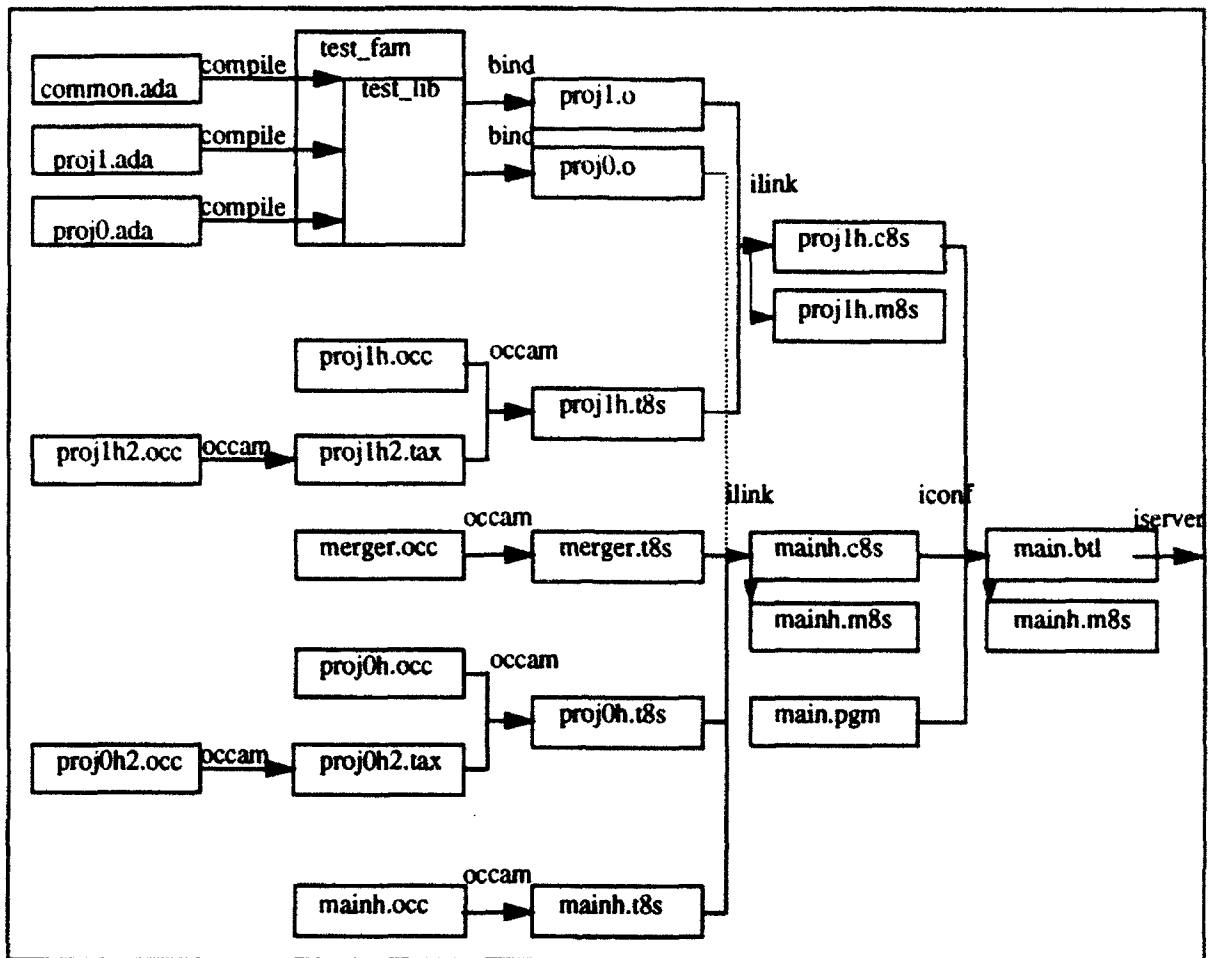
Figure 17: Diagram Of The Steps Involved In Program Development Using Alsys Ada On Transputers
