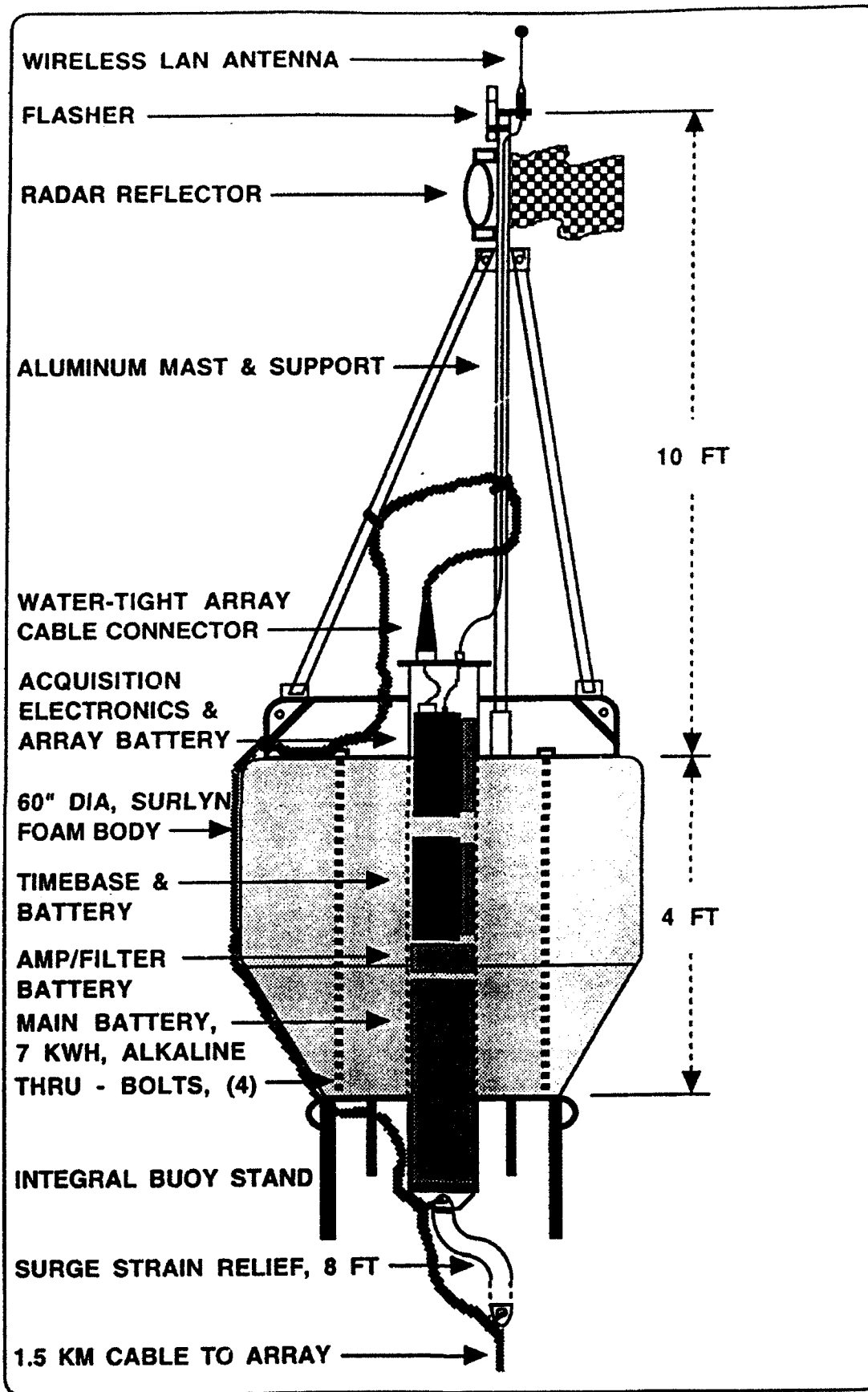
Figure 7. Cross section view of the Barents Sea telemetry buoy. The array cable was attached to the strain relief and brought up around the side of the buoy to a connector at the top of the central instrumentation tube.
