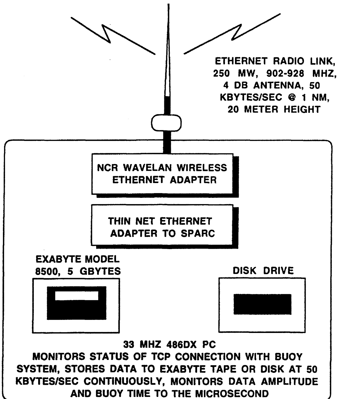
Figure 12. Barents Sea VLA data acquisition; shipboard system block diagram.
