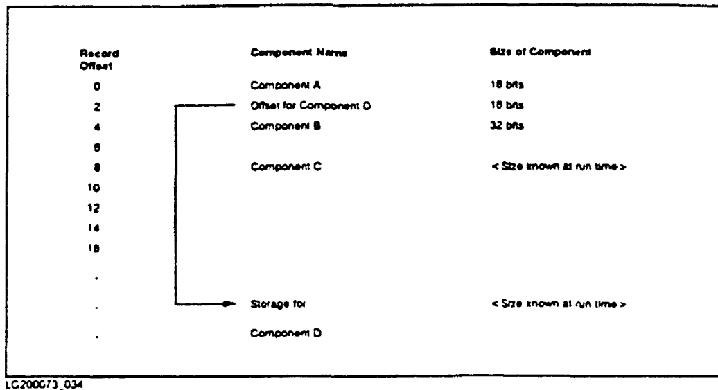
Figure 4-2. Record layout with an Indirect Component
