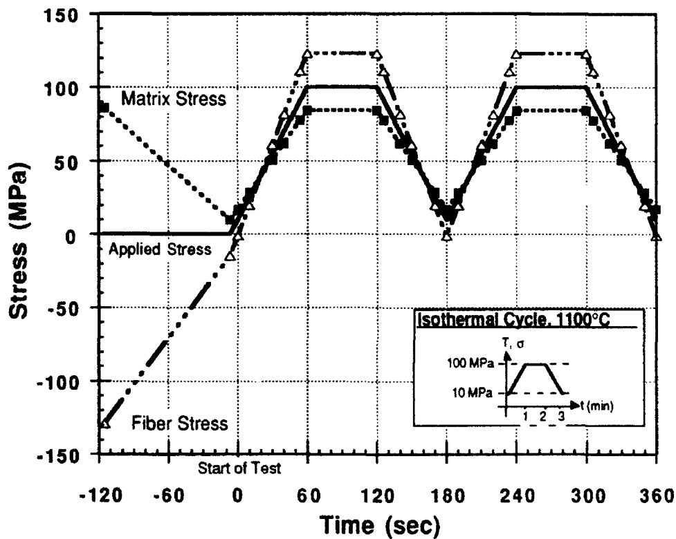
Figure 4-14. Axial stress states in the fiber and matrix plotted with applied stress for an isothermal fatigue cycle including a 60-sec hold at \sigma_{\max} . \sigma_{\max} = 100 MPa (14.5 ksi), R = 0.1
